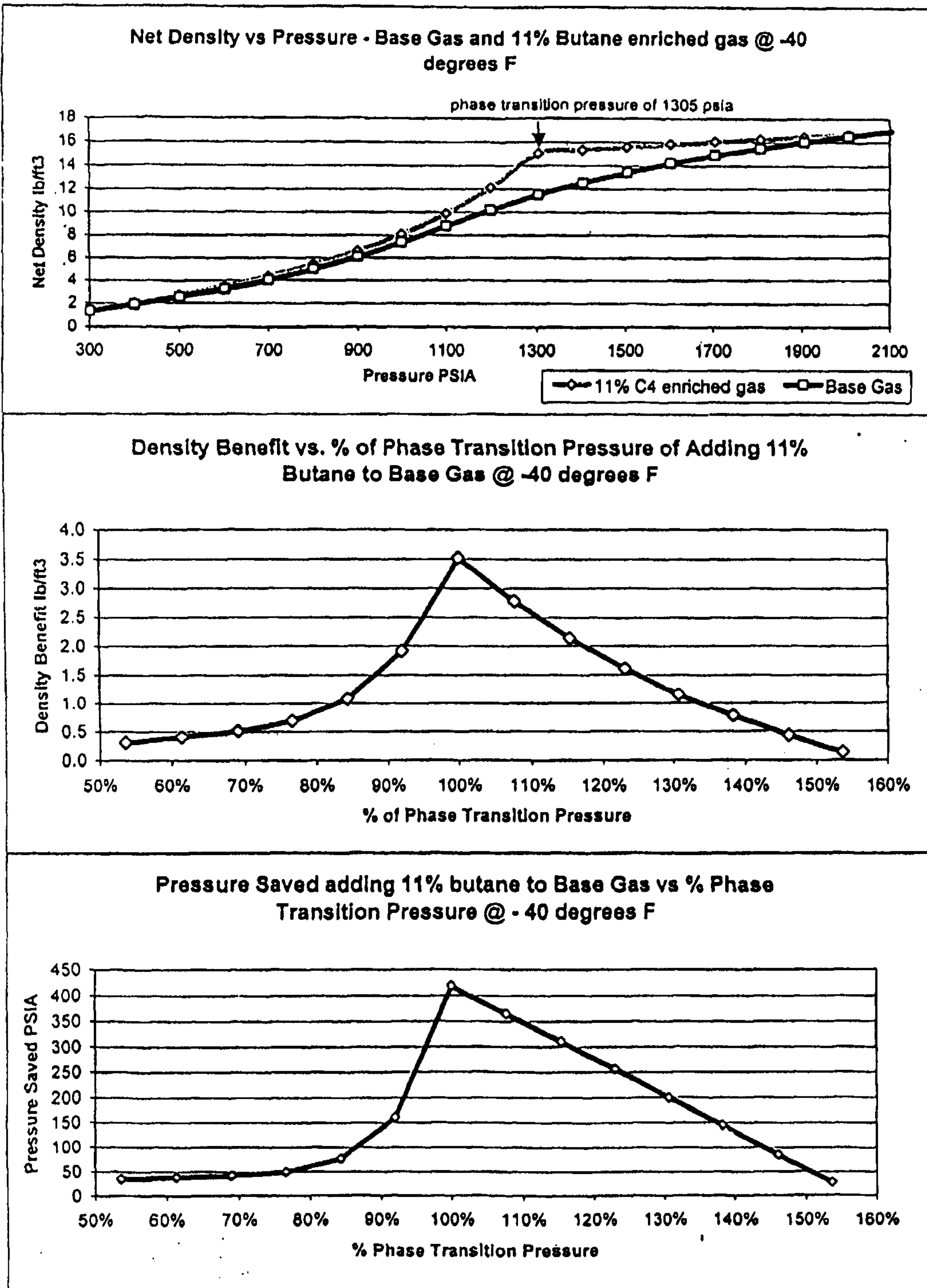
Figure # 10 - Gas Density with and without NGL addition vs. % of phase transition pressure
