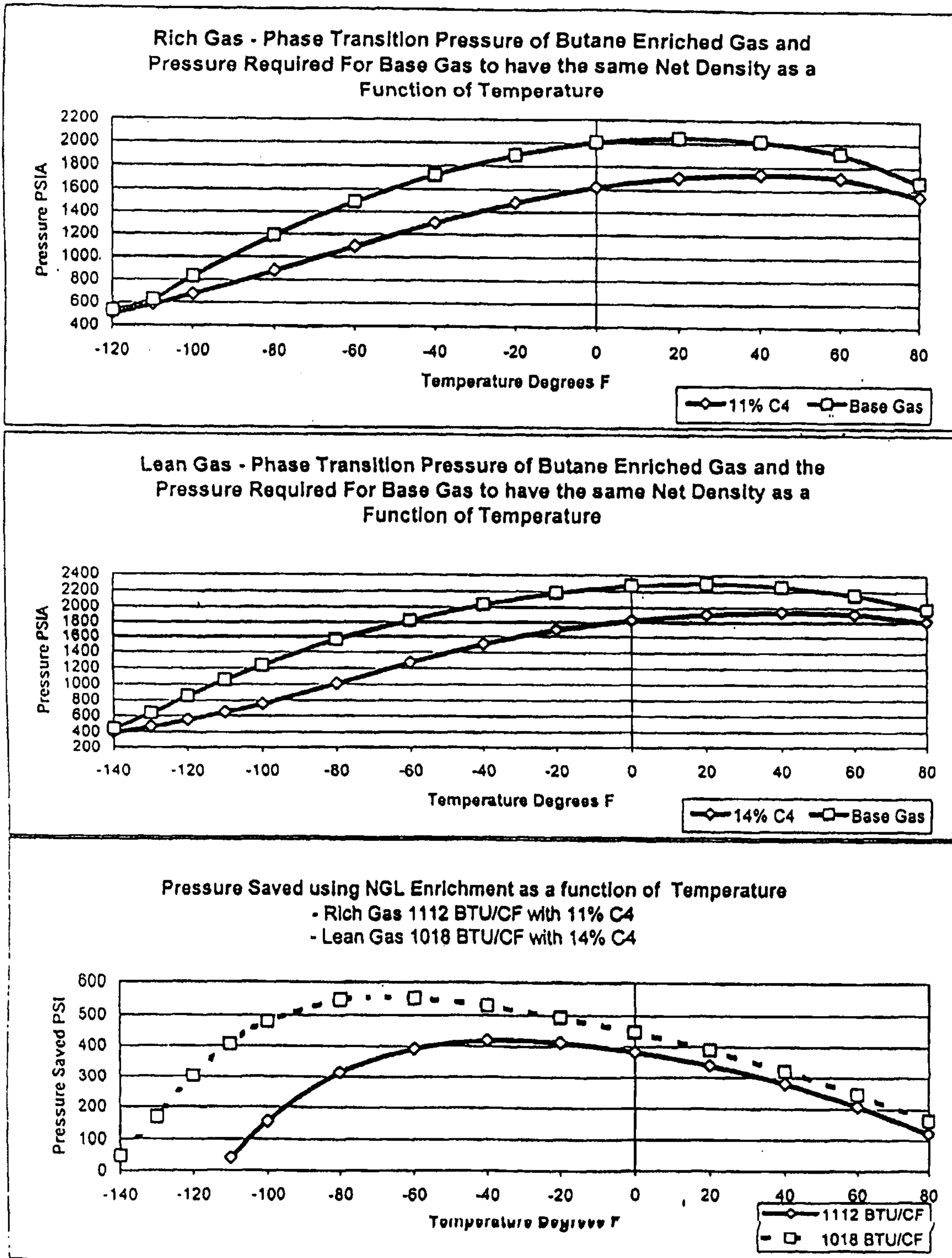
Figure # 9 - Pressure with and without NGL addition vs. Temperature
