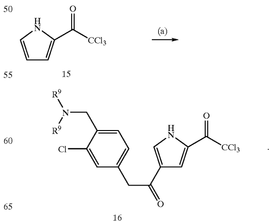
Scheme IV
