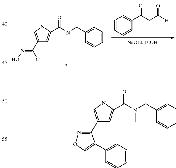
IIIA-22
