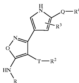
Compounds IV-A
