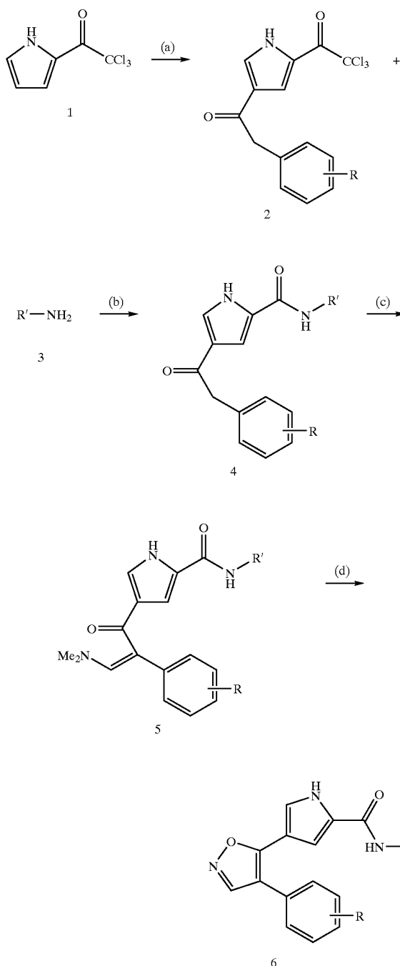
Scheme I
