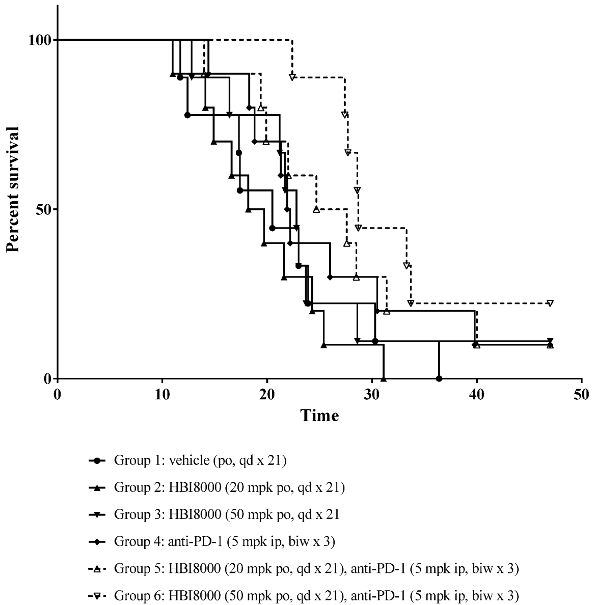
Fig. 3 Kaplan-Meier Survival Plot (Example 1, All groups)
