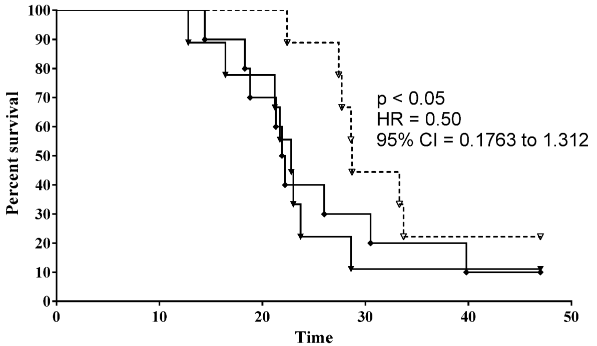
Fig. 4: Kaplan-Meier Survival Plot (Example 1, HBI-8000, 50 mpk groups)
