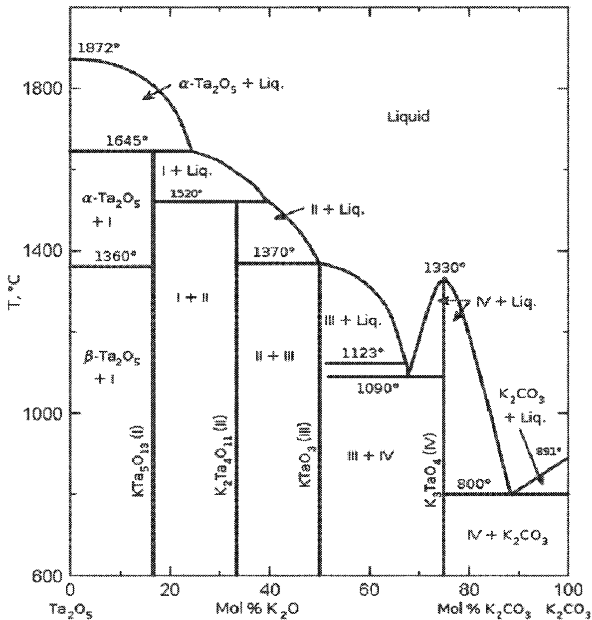
FIG. 2 (PRIOR ART)
