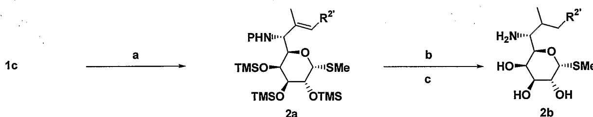
Scheme 2. General synthesis of lincosamine intermediate 2b.
