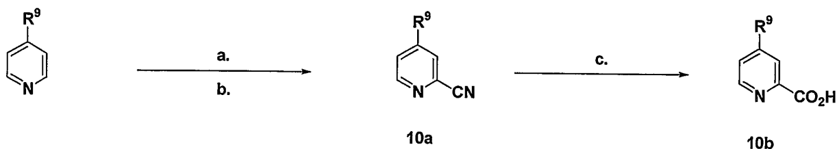
Scheme 10. General synthesis of substituted pyridin-2-yl carboxylic acids 10b .
