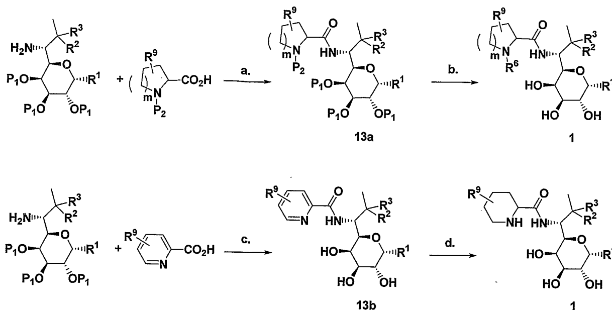
Scheme 13. General coupling and deprotection methods.
