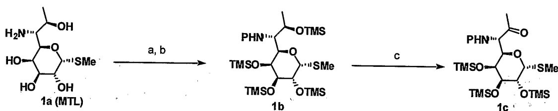
Scheme 1. General synthesis of lincosamine intermediate 1c.
