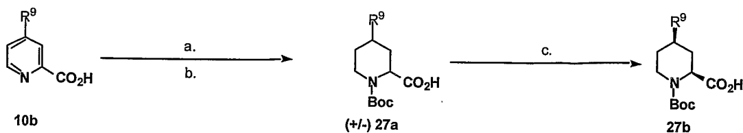
Scheme 27. General synthesis of racemic cis 4-substituted intermediates 27a and resolution to provide 2 S , 4 R R^9 intermediates 27b (a) PtO_2 , H_2 , H^+ (b) (Boc)_2O , ^iOH (c) i. chiral amine, recrystallization ii. H^+ .
