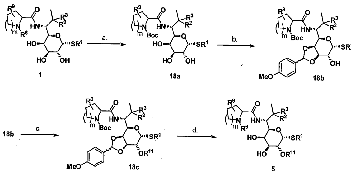
Scheme 27. General synthesis of racemic cis 4-substituted intermediates 27a and resolution to provide 2 S , 4 R R^9 intermediates 27b (a) PtO_2 , H_2 , H^+ (b) (Boc)_2O , ^iOH (c) i. chiral amine, recrystallization ii. H^+ .
