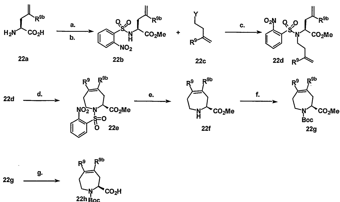
Scheme 22. a. H^+ , MeOH b. 2-nitrobenzenesulfonyl chloride, 2,4,6-collidine, dichloroethane c. CS_2CO_3 , TBABr, DMF, 22c (Y = Br, or OTs) or c. by Mitsunobu alkylation PPh_3 , Diisopropylazidodicarboxylate, 22c (Y = OH) d. Benzylidene[1,3-bis(2,4,6-trimethylphenyl)-2-imidazolidinylidene] dichloro-(tricyclohexylphosphine)ruthenium e. organic base (7-methyl,1,5,7-triazabicyclo[4.4.0]dec-5-ene), thiophenol f. (Boc) _2 O, TEA g. Aq. LiOH, Dioxane.
