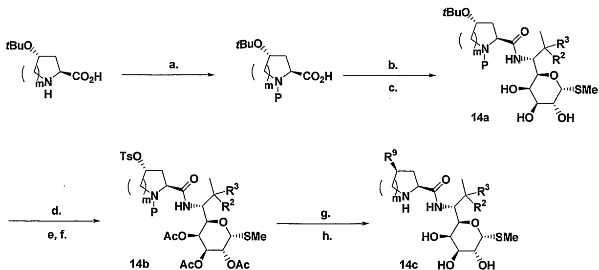
Scheme 14. General synthesis of 4-thioetherlincosamides 14c.
