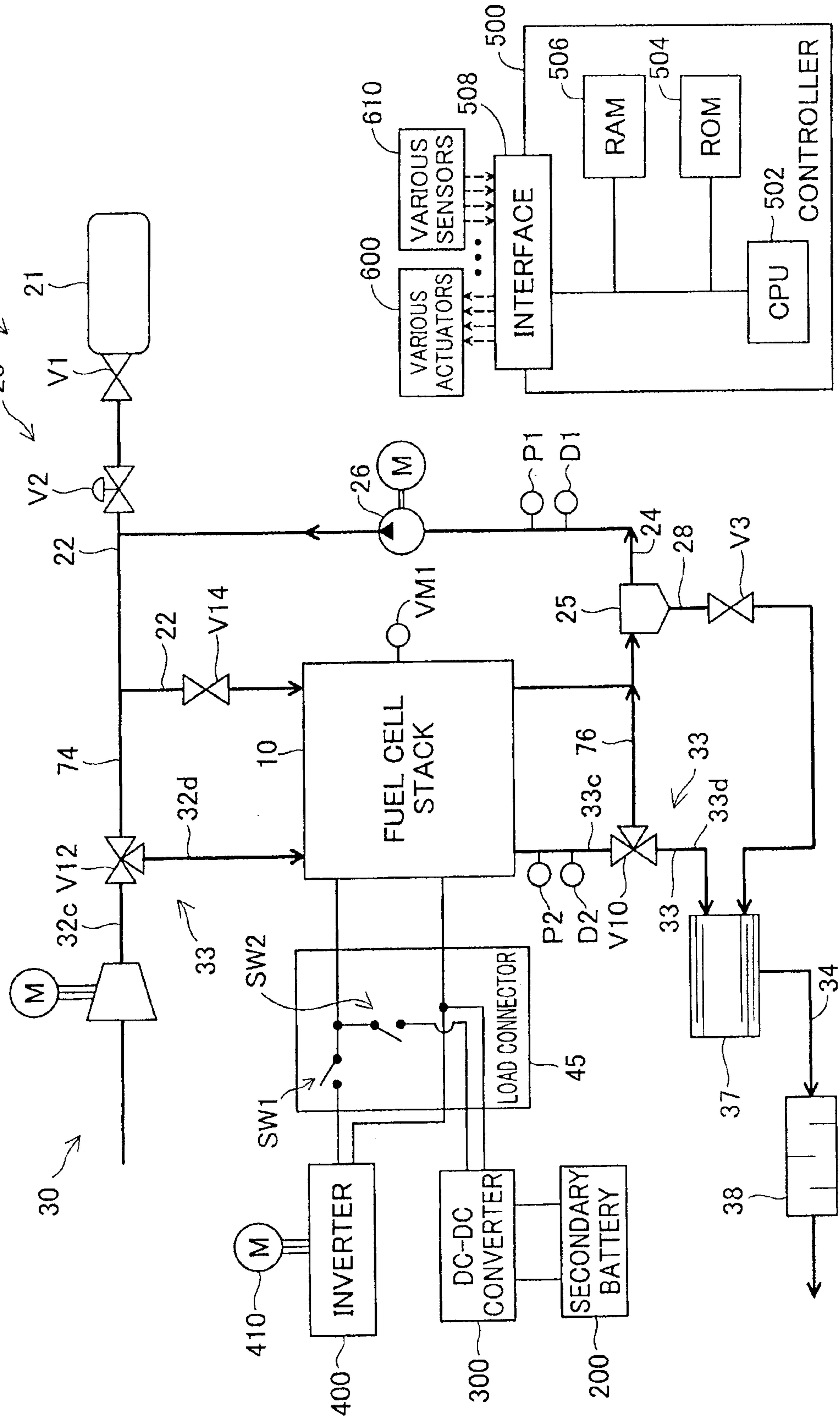
Fig.14 120a FUEL CELL SYSTEM
