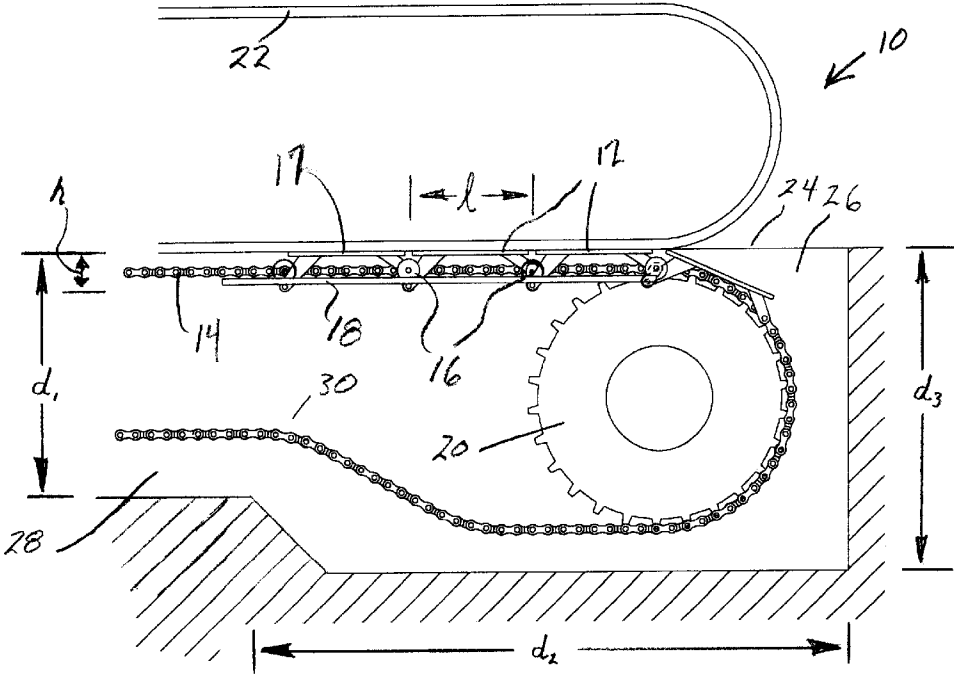
Fig. 2 (PRIOR ART)
