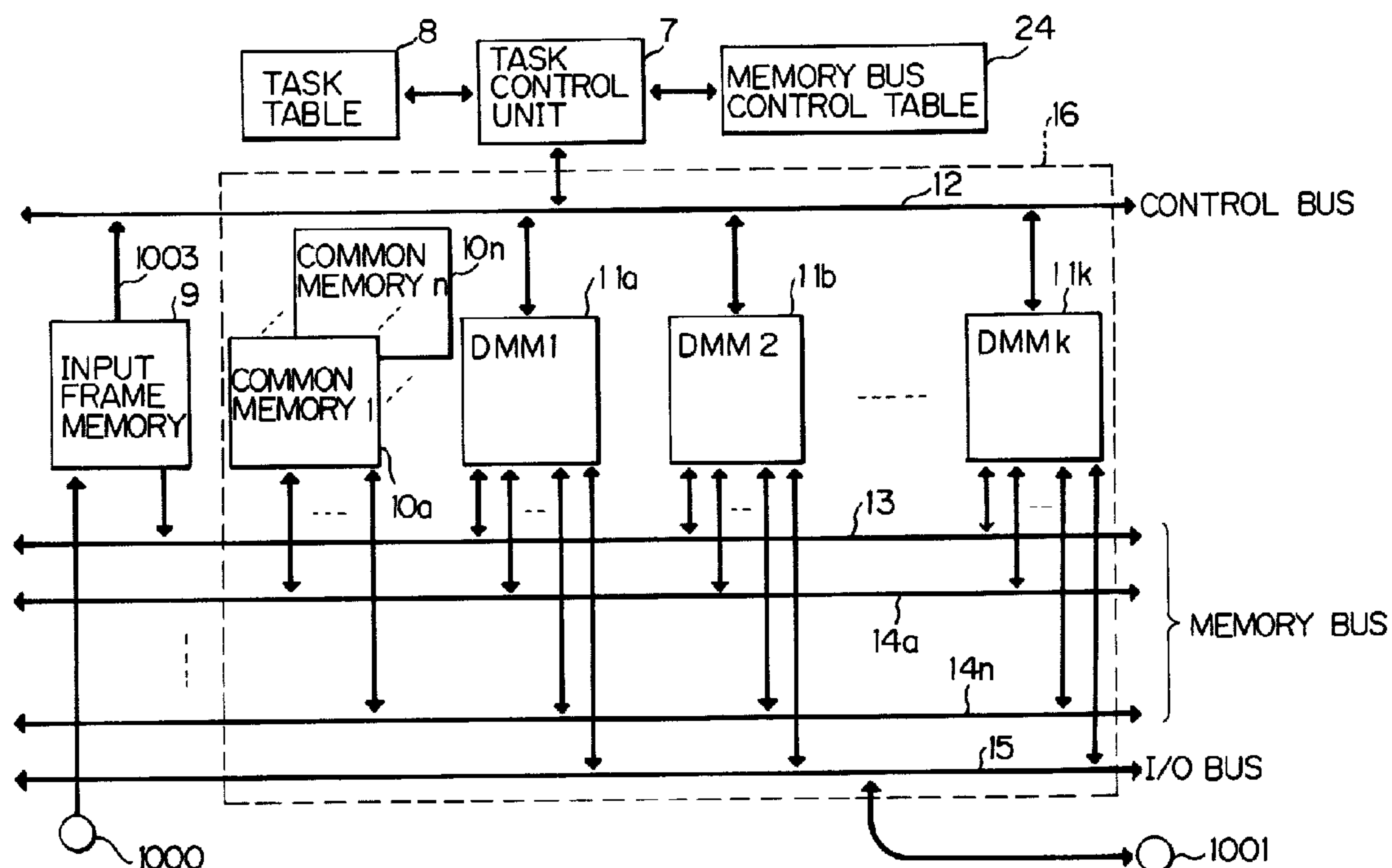
SINGLE-DMM MODULE ARRANGEMENT OF MULTIPROCESSOR TYPE TIME VARYING IMAGE ENCODING SYSTEM
