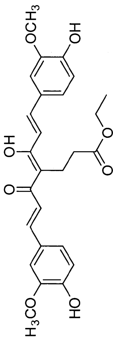
5-Hydroxy-7-(4-hydroxy-3-methoxyphenyl)-4-[3-(4-hydroxy-3-methoxyphenyl)-acryloyl]-hepta-4,6-dienoic acid ethyl ester
