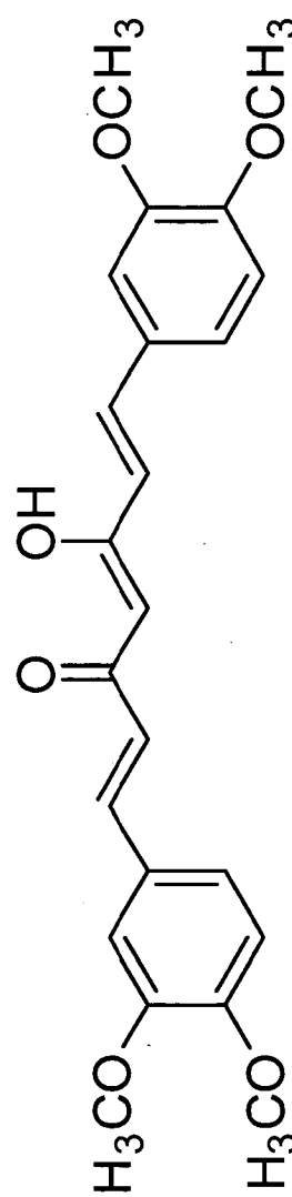
1,7-Bis-(3,4-dimethoxyphenyl)-5-hydroxy-hepta-1,4,6-trien-3-one (dimethyl curcumin)
