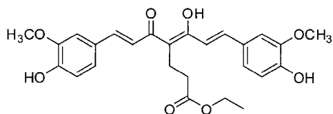
5-Hydroxy-7-(4-hydroxy-3-methoxyphenyl)-4-[3-(4-hydroxy-3-methoxyphenyl)-acryloyl]-hepta-4,6-dienoic acid ethyl ester
