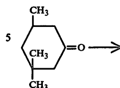
Dihydroisophorone
