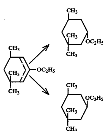
Enol Ether
