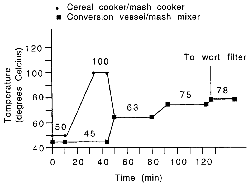
Figure 1 Brewing diagram
