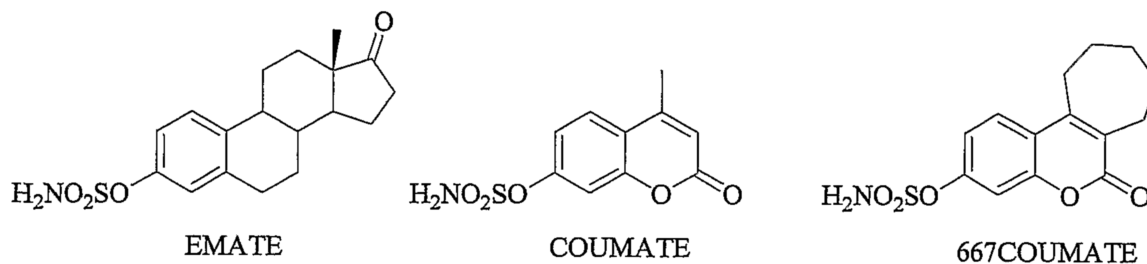
Structures of the steroid sulphatase inhibitors EMATE, COUMATE and 667COUMATE.
