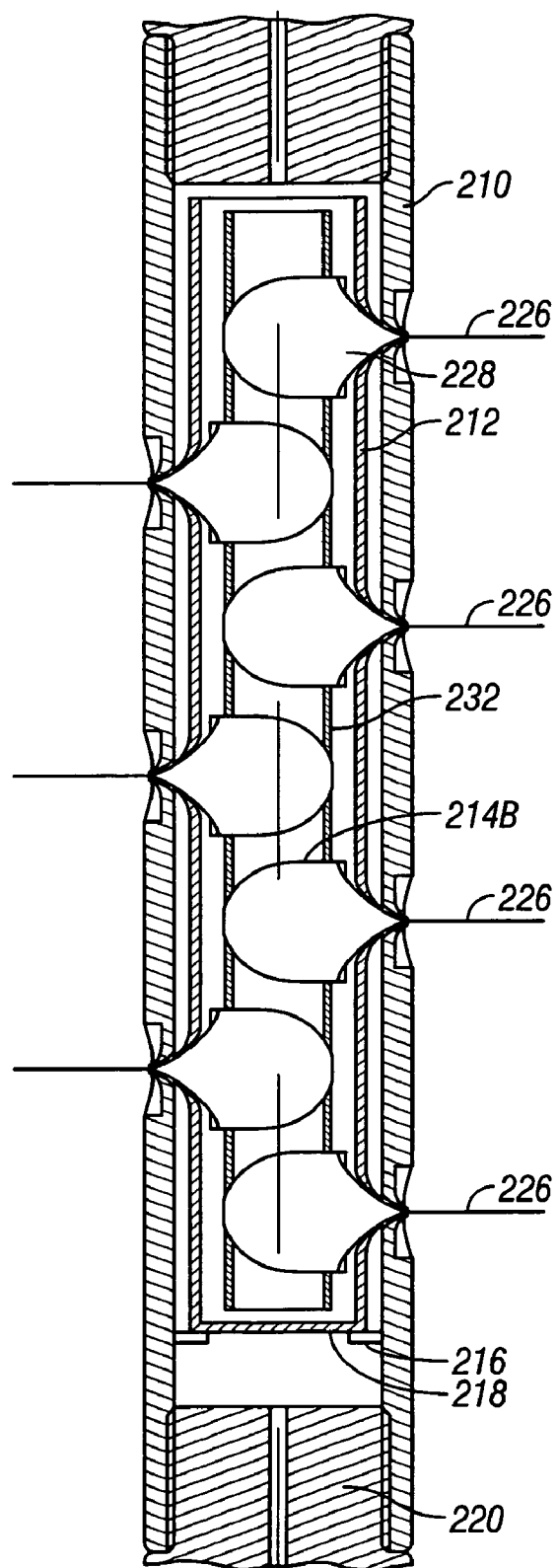
FIG. 4 (Prior Art)
