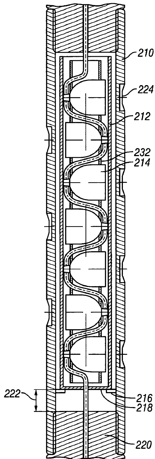
FIG. 3 (Prior Art)
