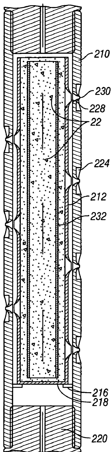
FIG. 5 (Prior Art)
