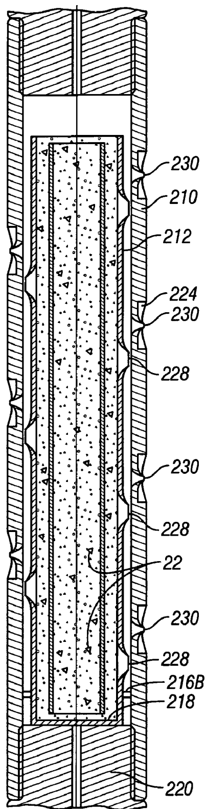
FIG. 6 (Prior Art)
