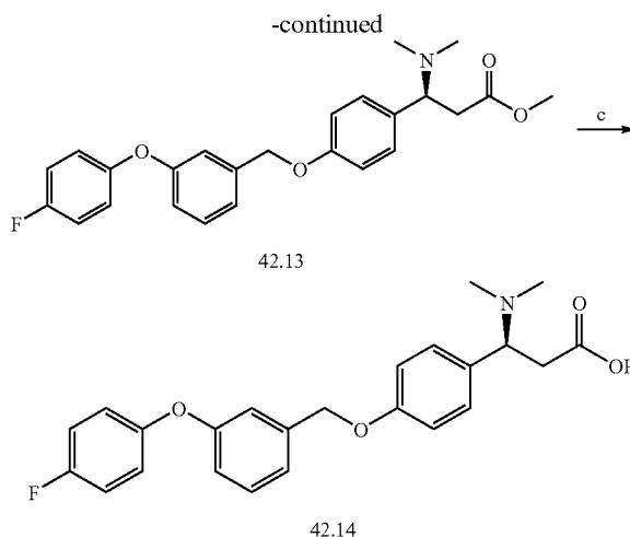
Scheme 42.3. a. TFA, DCM, r.t., 1 h; b. formaldehyde, NaBH(OAc) 3 , AcOH, DMF, r.t., overnight; c. LiOH/THF, MeOH, and water, r.t., 2 h.
