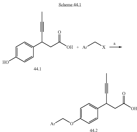
Scheme 44.1. a. NaOH, EtOH, water, r.t., 3 h (X = Br, Cl).
