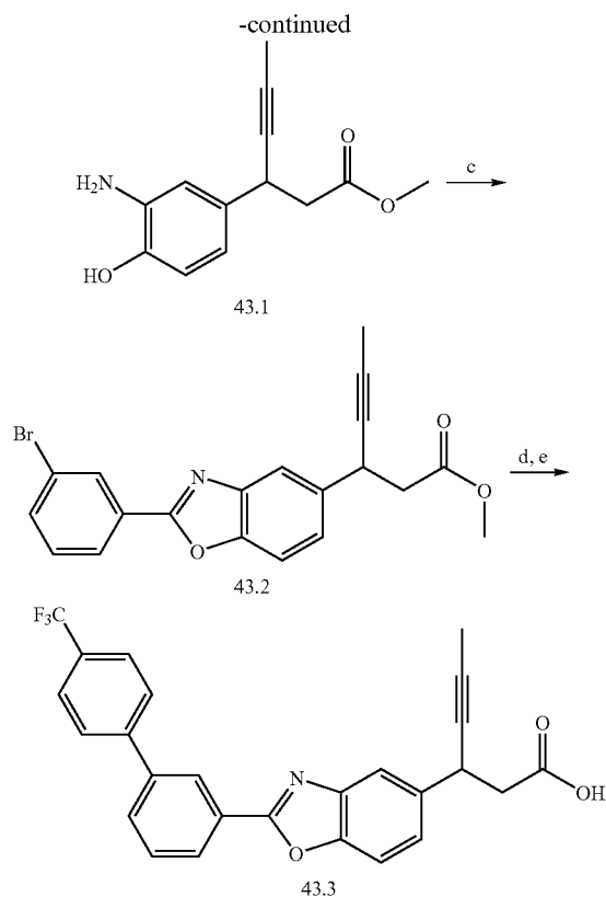
Scheme 43.1. a. \text{HNO}_3 , HOAc, 80^\circ\text{C} , 3 h; b. \text{SnCl}_2 , EtOAc/EtOH, 70^\circ\text{C} , 3 h; c. 3-bromobenzaldehyde, DDQ, DMF, r.t. 2 h; d. 4-trifluoromethylbenzeneboronic acid, \text{Pd}(\text{PPh}_3)_4 , DME, \text{Na}_2\text{CO}_3 , 80^\circ\text{C} , 14 h; e. LiOH/THF, MeOH, and water, r.t., 2 h.
