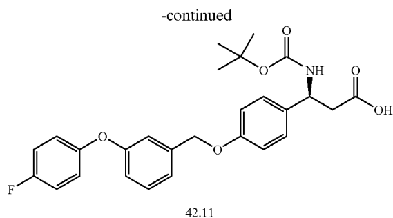
Scheme 42.2. a. TMSCHN 2 , MeOH, benzene, r.t., 1 h; b. K 2 CO 3 , DMF, r.t., overnight; c. LiOH/THF, MeOH, and water, r.t., 2 h.
