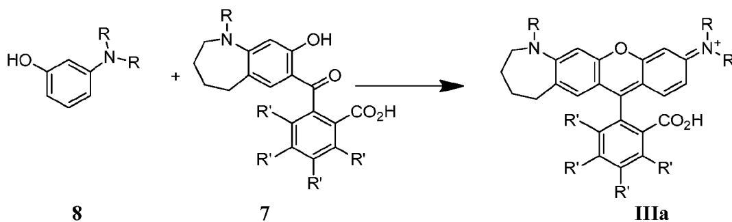
Scheme 6
