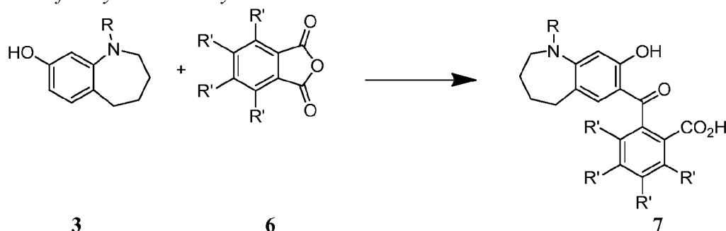
Scheme 5
