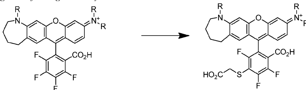
Scheme 7
