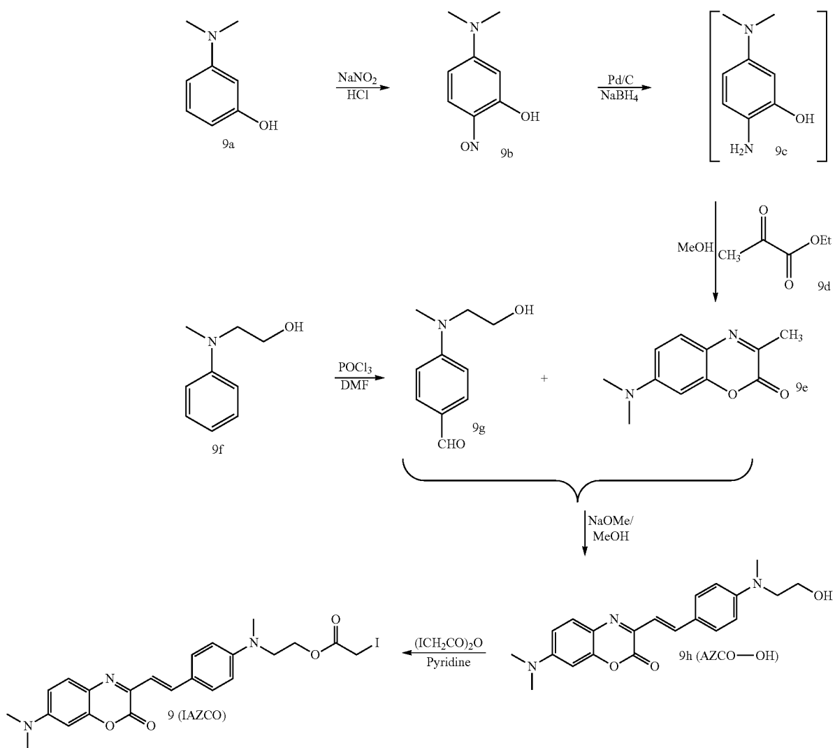
Scheme VIII
