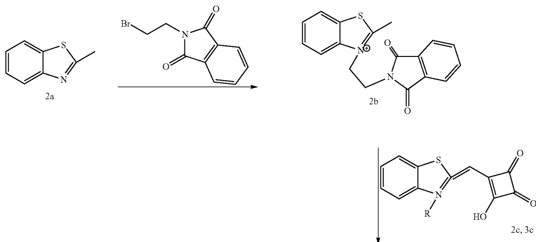
Scheme II
