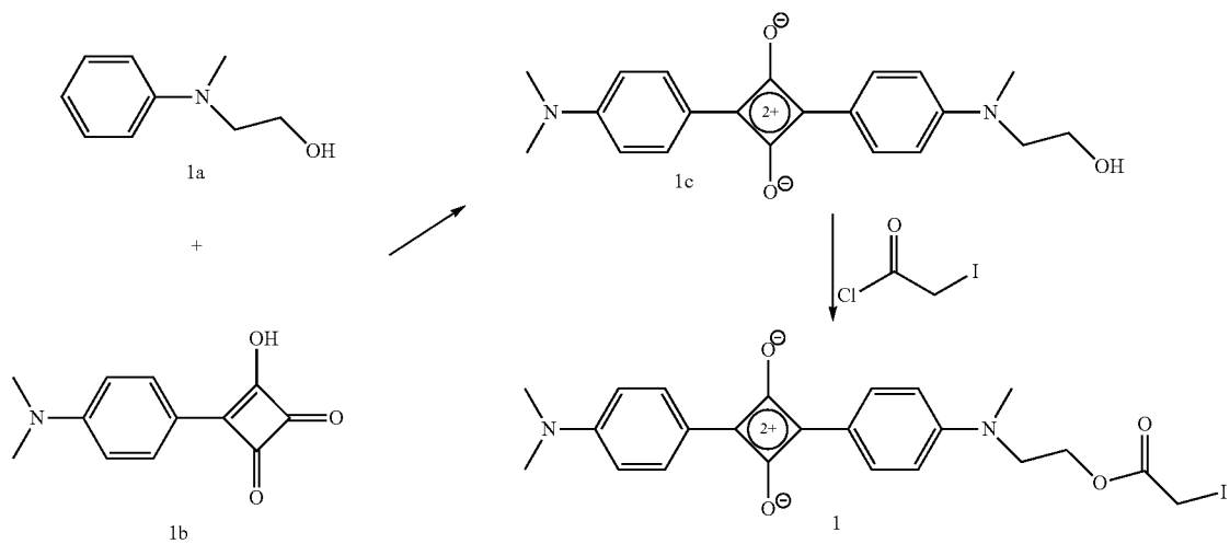
Scheme I
