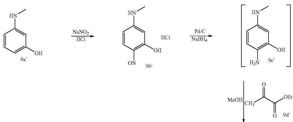
Scheme VIIIa
