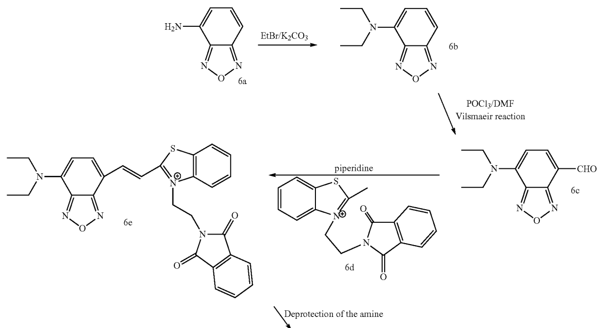
Scheme V
