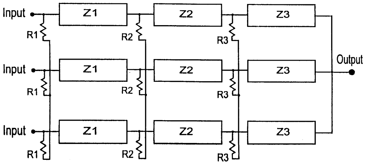
FIG. 3 (Prior Art)
