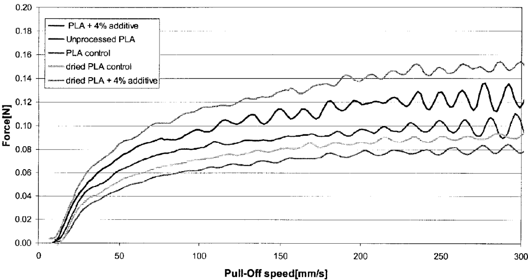
Figure 2: Rheotens Analysis of Dried PLA samples
