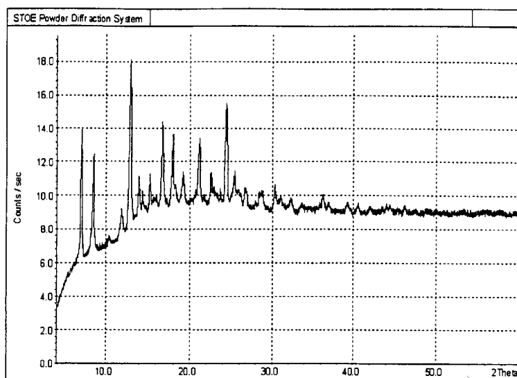
Fig.1: powder X-ray diffraction pattern of Mn(III)salen (compound (2)), obtained from Example 1.
