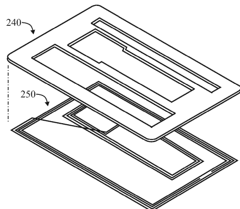
FIG. 2B Selectively-Deposited Shielding Layer
