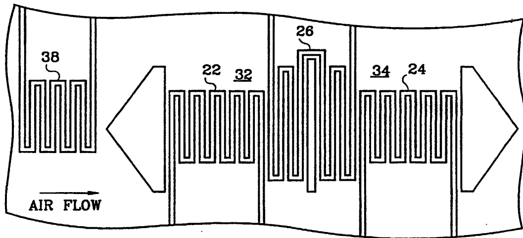
Fig. 2 (PRIOR ART)
