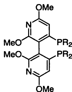
P-Phos (Chan)
