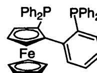
(Knochel)
