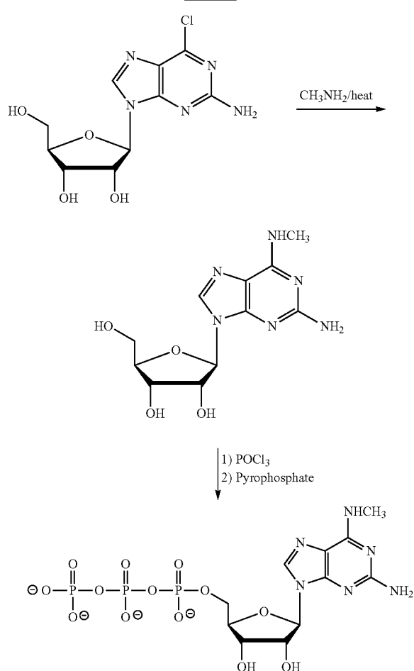
Scheme 8
