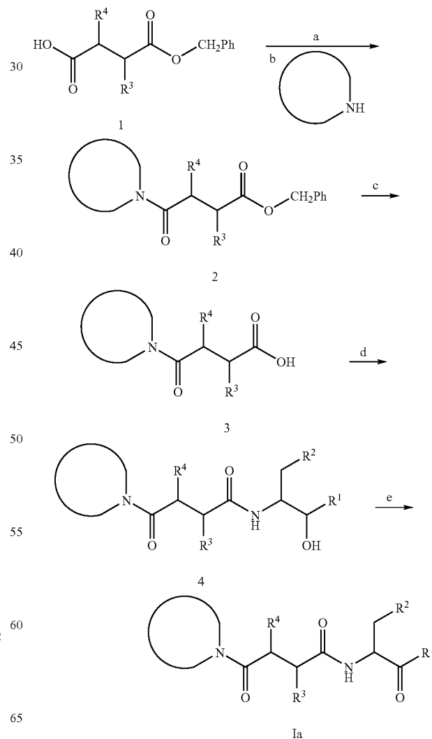
Scheme I
