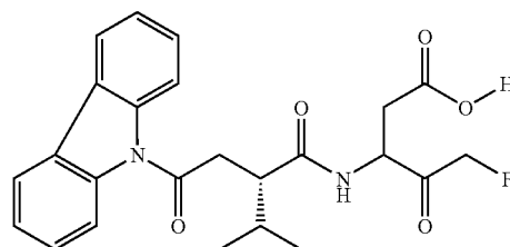
[3S/R(2S)]-3-[2-(2-Carbazol-9-yl-2-oxo-ethyl)-3-methyl-butyrylamino]-5-fluoro-4-oxo-pentanoic acid
