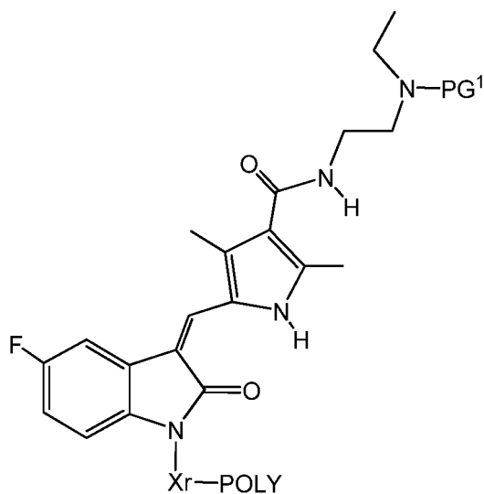
(Formula I-C-PG 1 )
