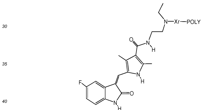
(Formula I-C)
