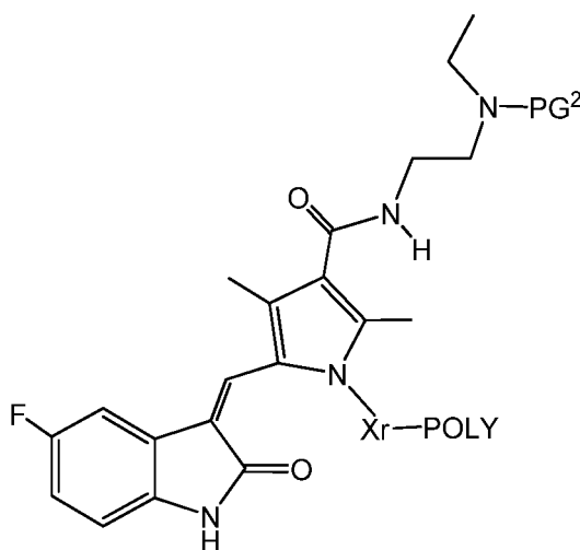
(Formula I-C-PG 2 )
