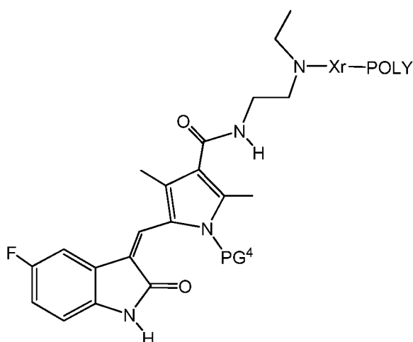
(Formula I-C-PG 4 )
