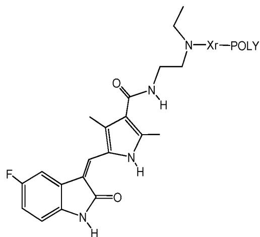
(Formula I-C)
