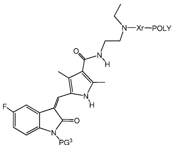
(Formula I-C-PG 3 )
