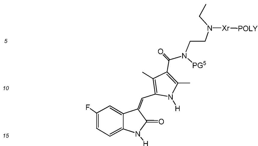
(Formula I-C-PG 5 )
