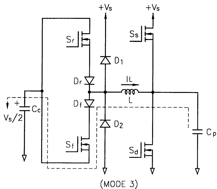
FIG. 3C (PRIOR ART)
