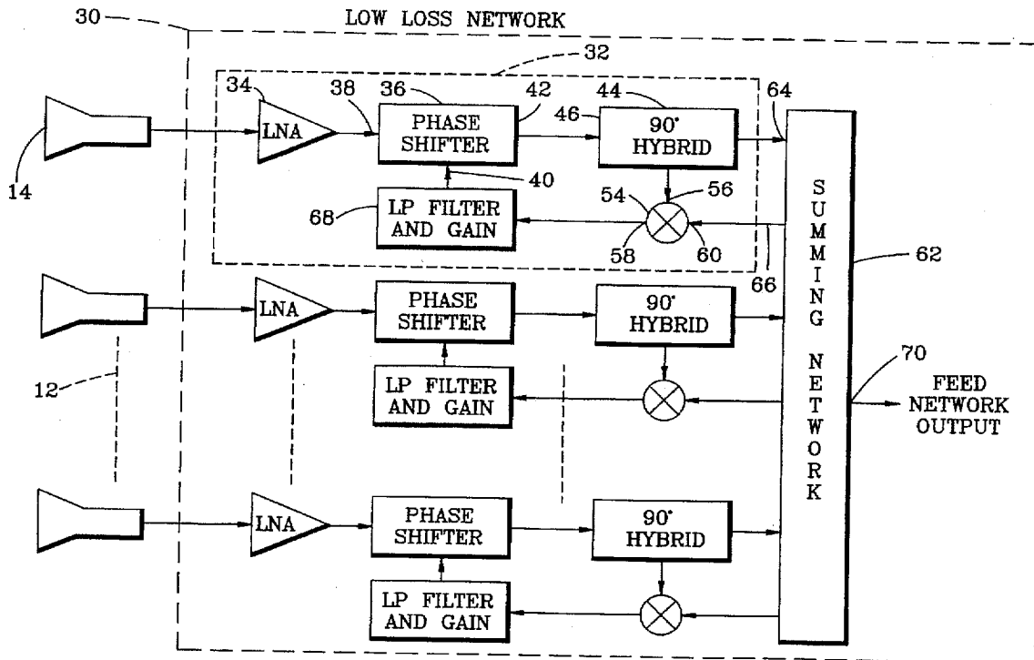
COHERENT PHASING OF THE OUTPUT OF THE ENSEMBLE OF FEEDS IS ACCOMPLISHED WITH THE PHASE CONTROL LOOPS.
