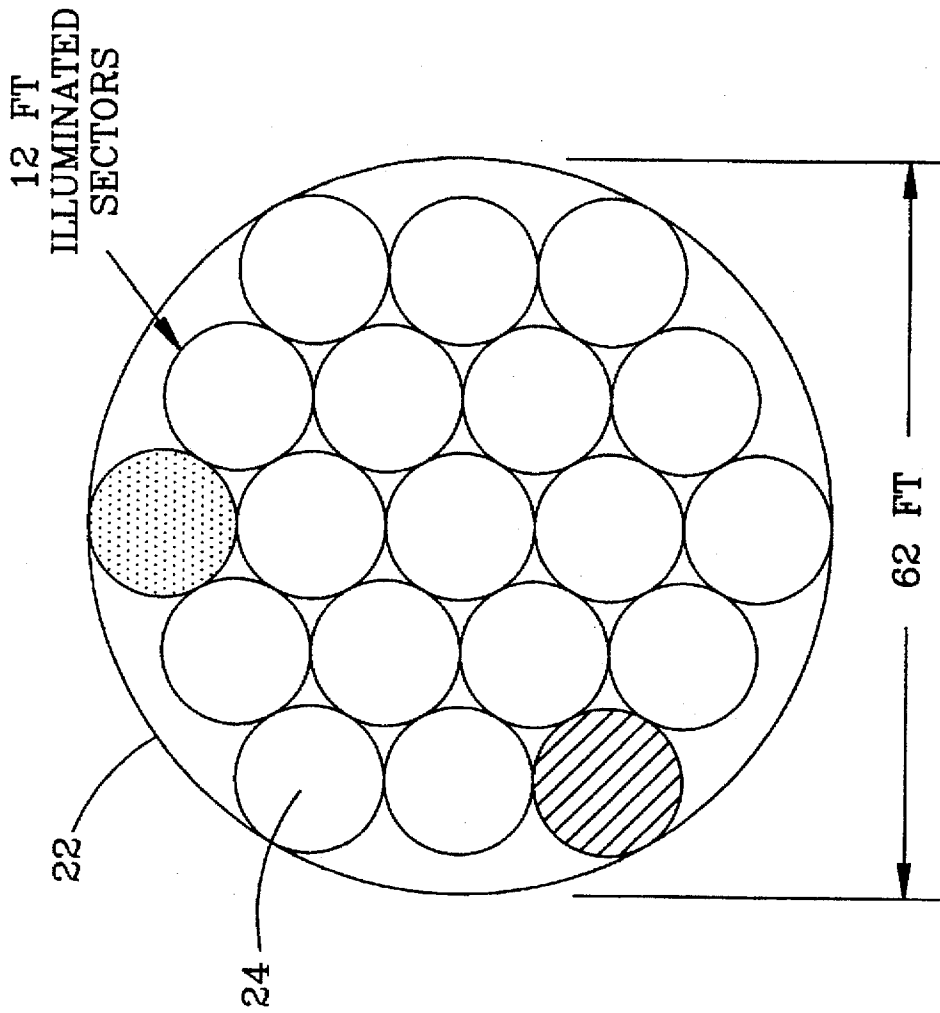
CIRCULAR APERTURE ILLUMINATED IN 12 FOOT DIAMETER SECTORS
