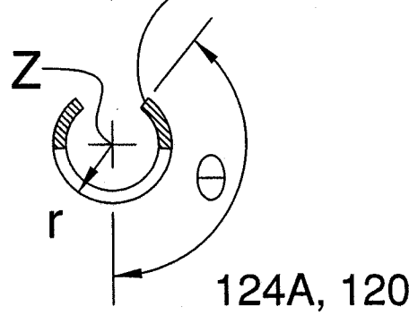
FIG. 6C SECTION F-F
