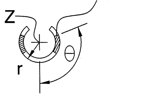
FIG. 6B SECTION E-E
