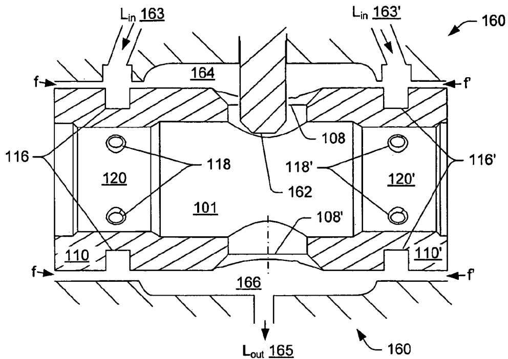
Fig. 1C (Prior Art)
