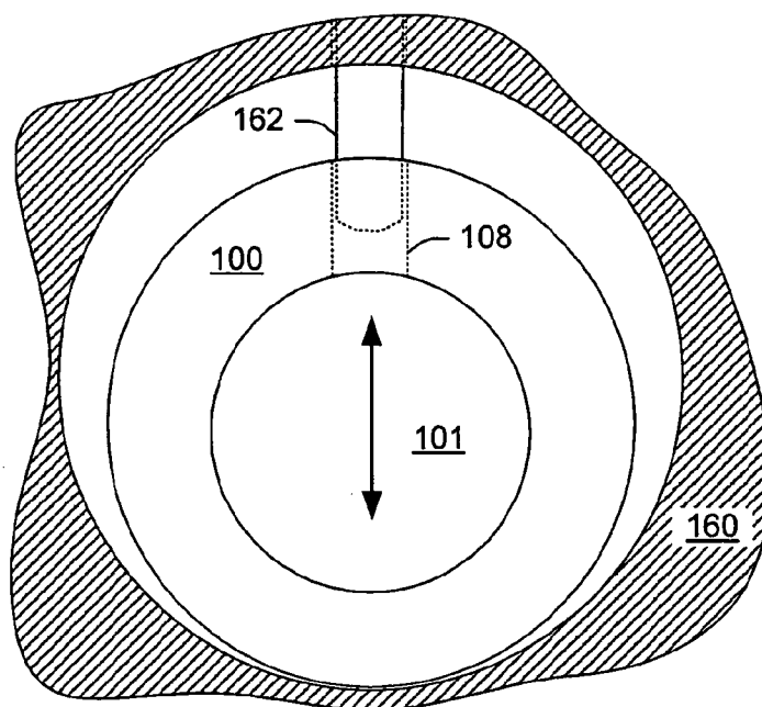
Fig. 1C (Prior Art)
