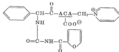
7- D- \alpha -[3-(2-furoyl)ureido]phenylacetamido -3-(1-pyridylmethyl)-3-cephem-4-carboxylic acid betaine
