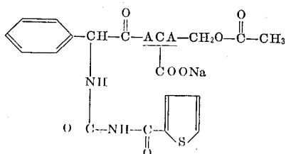
Sodium 7-{D- \alpha -[3-(2-thienoyl)ureido]phenylacetamido}cephalosporanate
