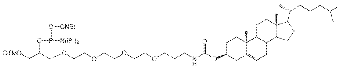
Cholesteryl-TEG Phosphoramidite
