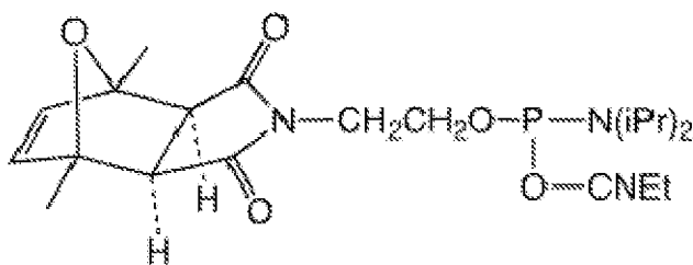
5'-Maleimide-Modifier Phosphoramidite
