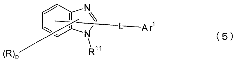
[Chemical Formula 8]
