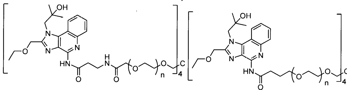
Compound 2
