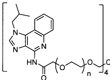
Compound 15
