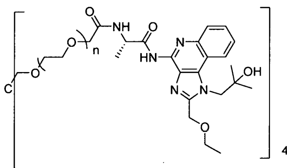
Compound 7
