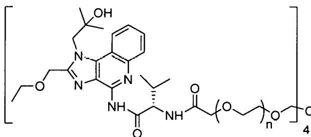
Compound 8
