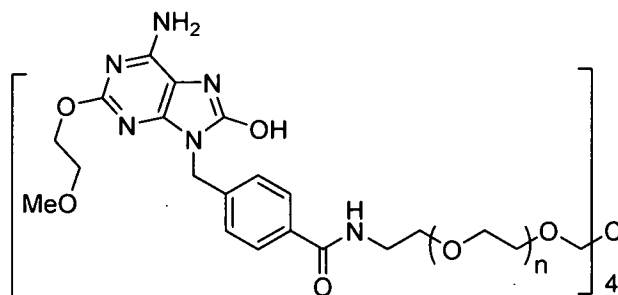
Compound 16
