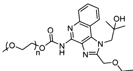
Compound 11
