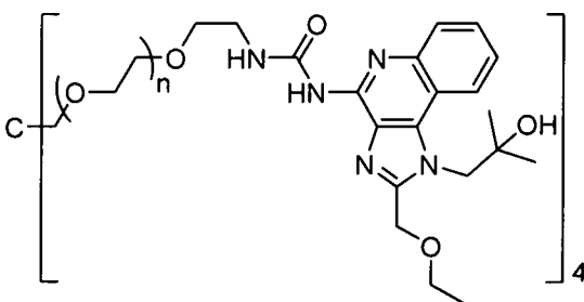
Compound 13
