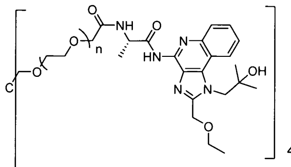
Compound 7
