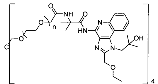
Compound 10
