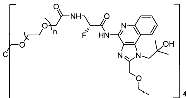
Compound 4
