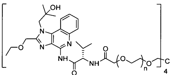
Compound 8
