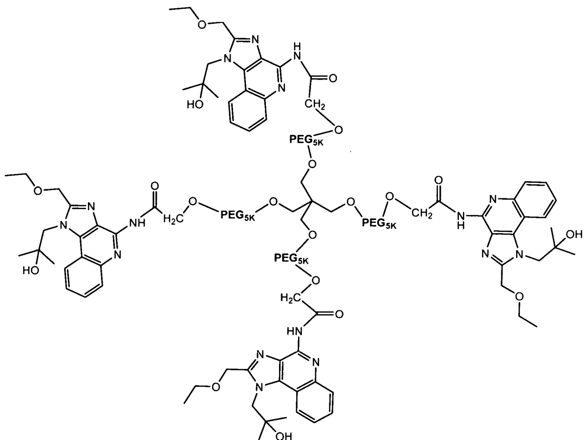
Compound 1
