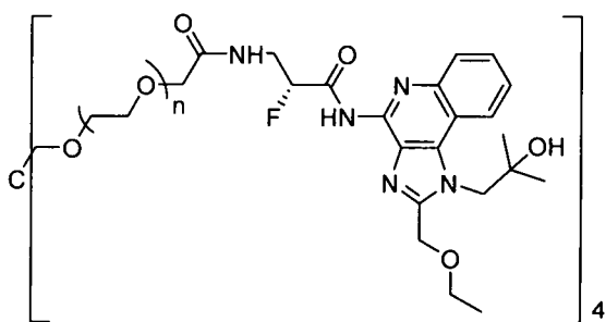
Compound 4
