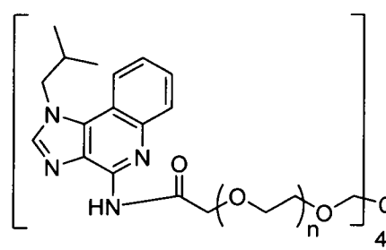
Compound 14
