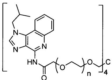
Compound 15
