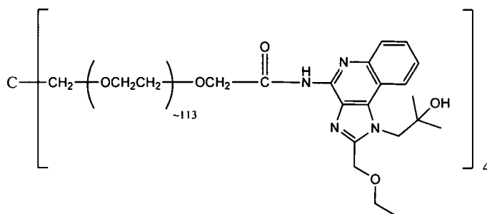
"4-arm-PEG20kD-CM-N-R848"
