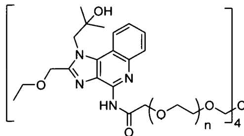
Compound 5
