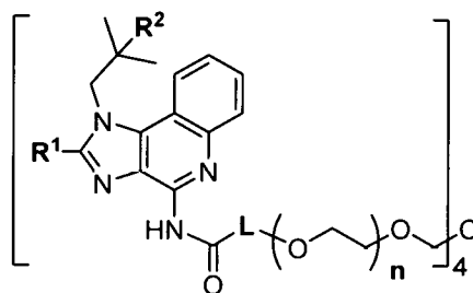
(Formula III)
