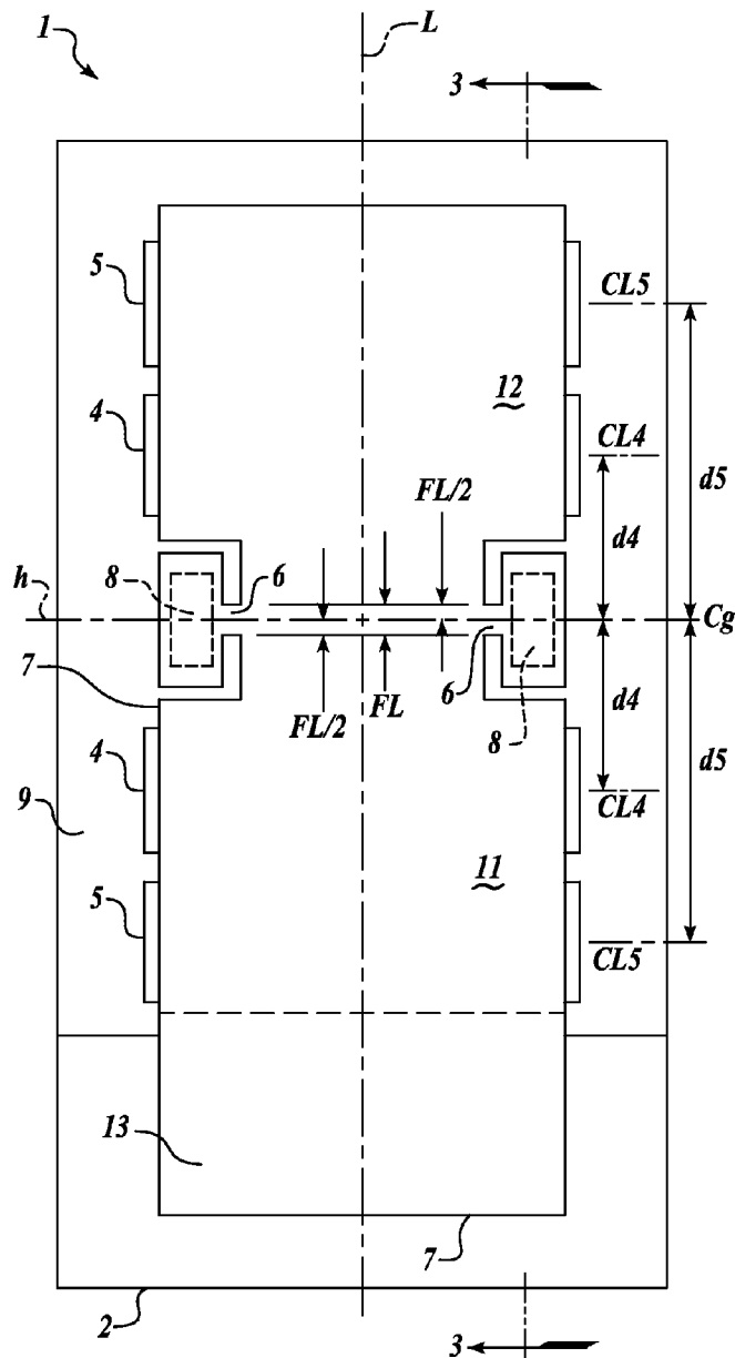
FIG.2 (PRIOR ART)
