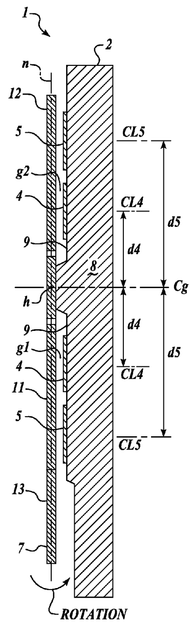
FIG.3 (PRIOR ART)
