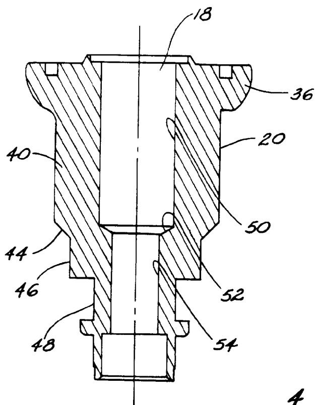
Fig. 2 PRIOR ART
