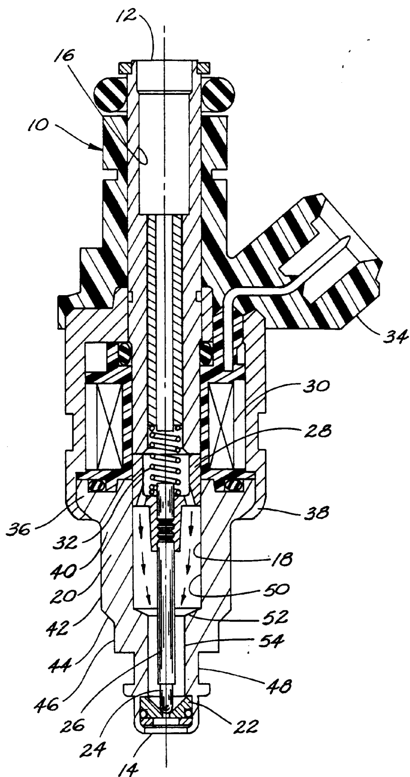
Fig. 1 PRIOR ART
