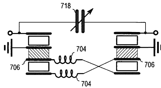
Fig. 12B Bandpass Filter Fixed . Tuned zero
