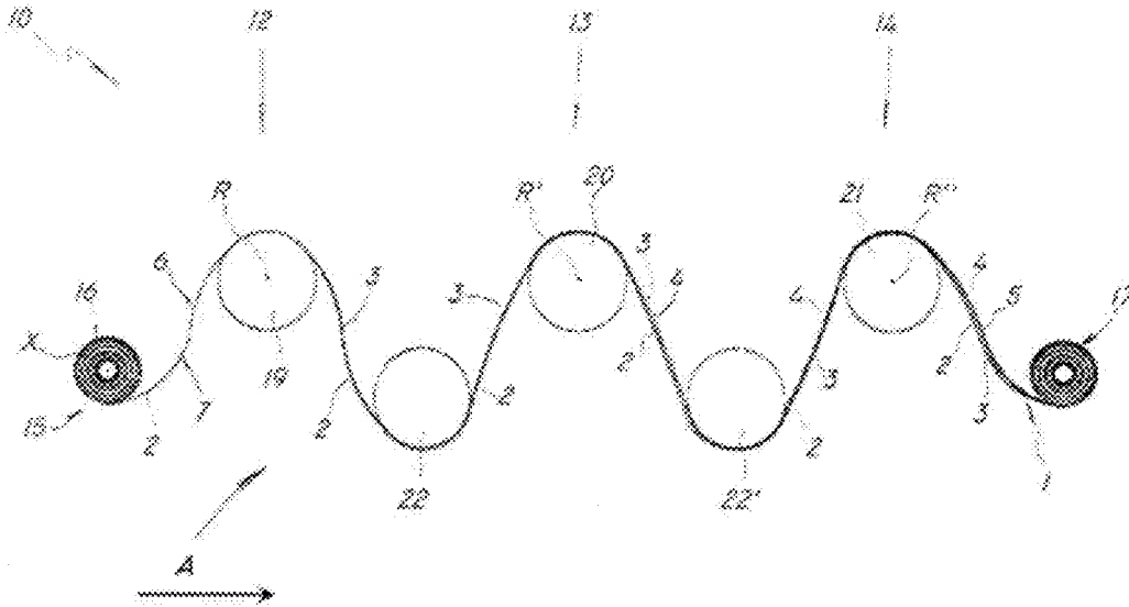
FIG. 3 (FIG 3 of U.S. Pat 8,852,369 from Prior Art)
