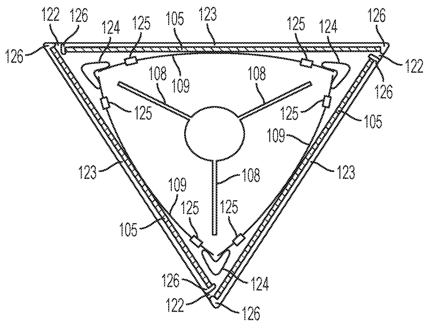
SECTION F-F
