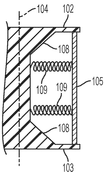
SECTION B-B
