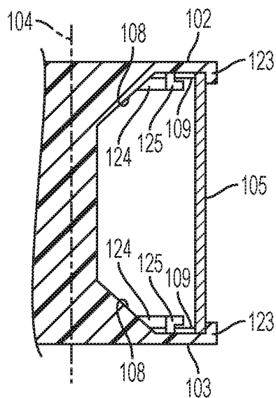
SECTION E-E
