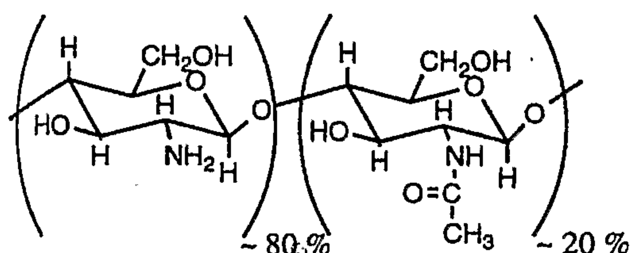
Chitosan
