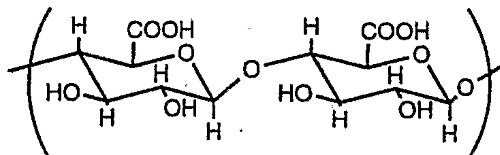
Alginic acid
