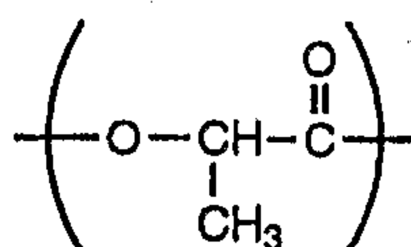
Poly(lactic acid)
