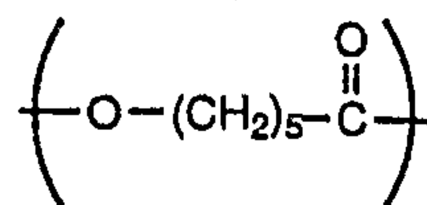
Polycaprolactone
