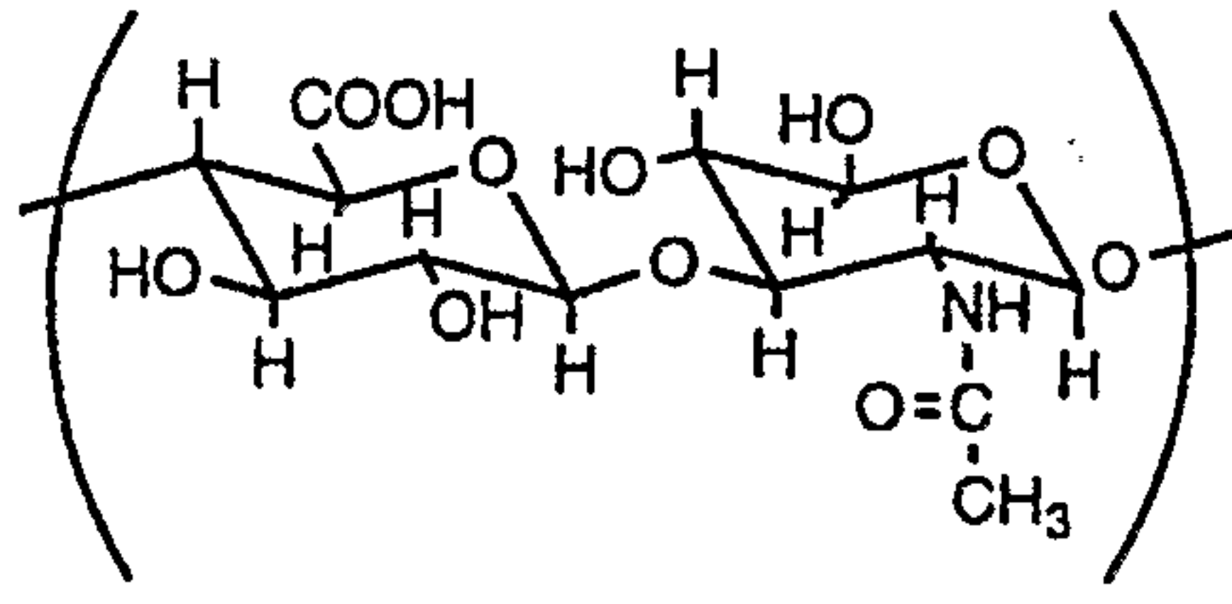
Hyaluronic acid
