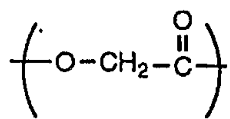
Poly(glycolic acid)
