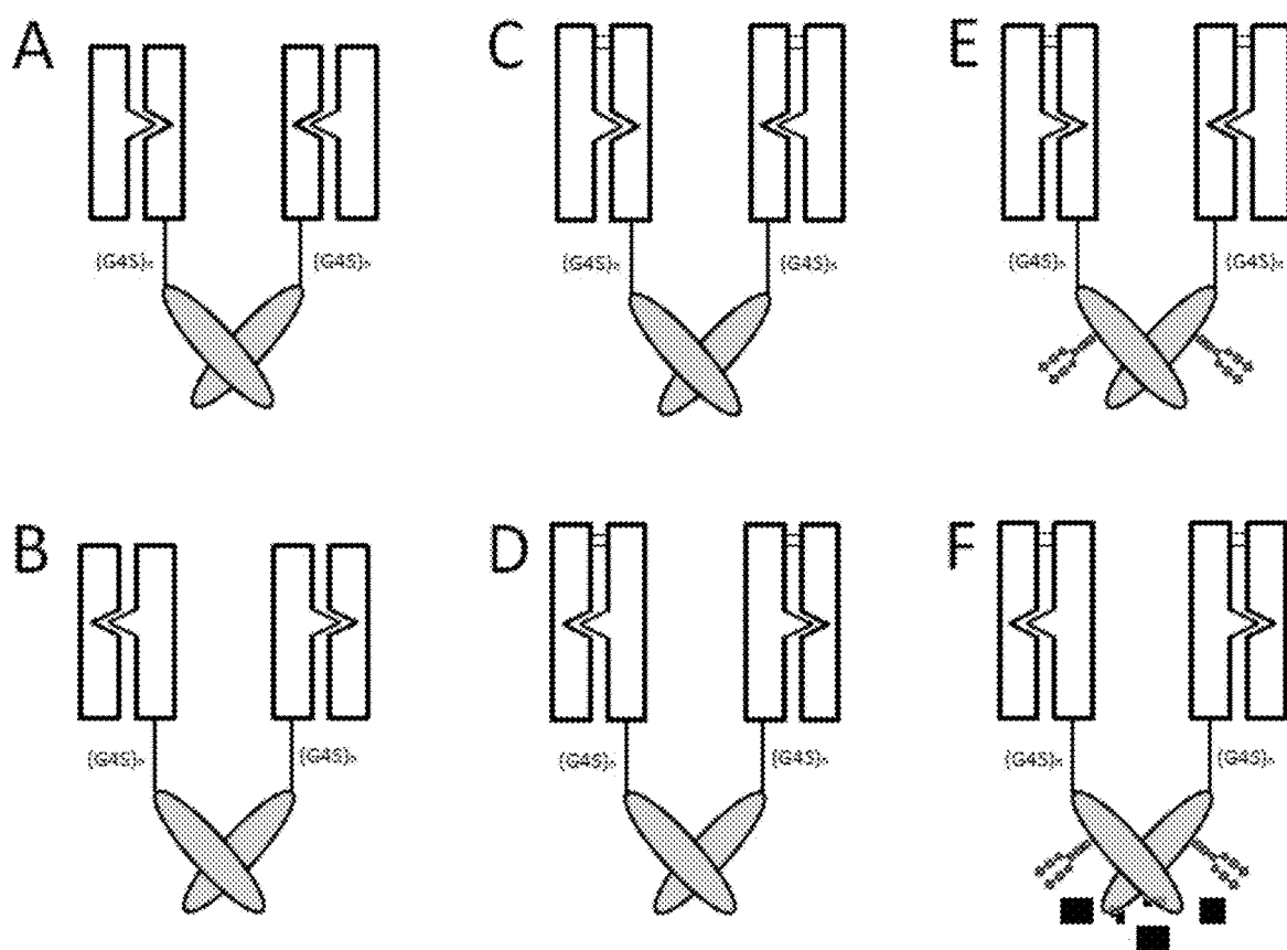
Figure 1 – Designs of knob-in-hole (Fc/Fc)-GDF15 molecules
