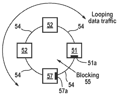
FIG. 4 (Prior Art)
