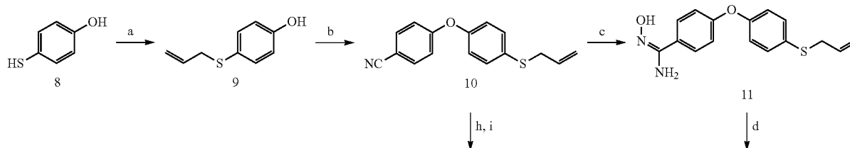
Scheme 1. Syntheses of the inhibitors 4, 5, 6 and 7 a .
