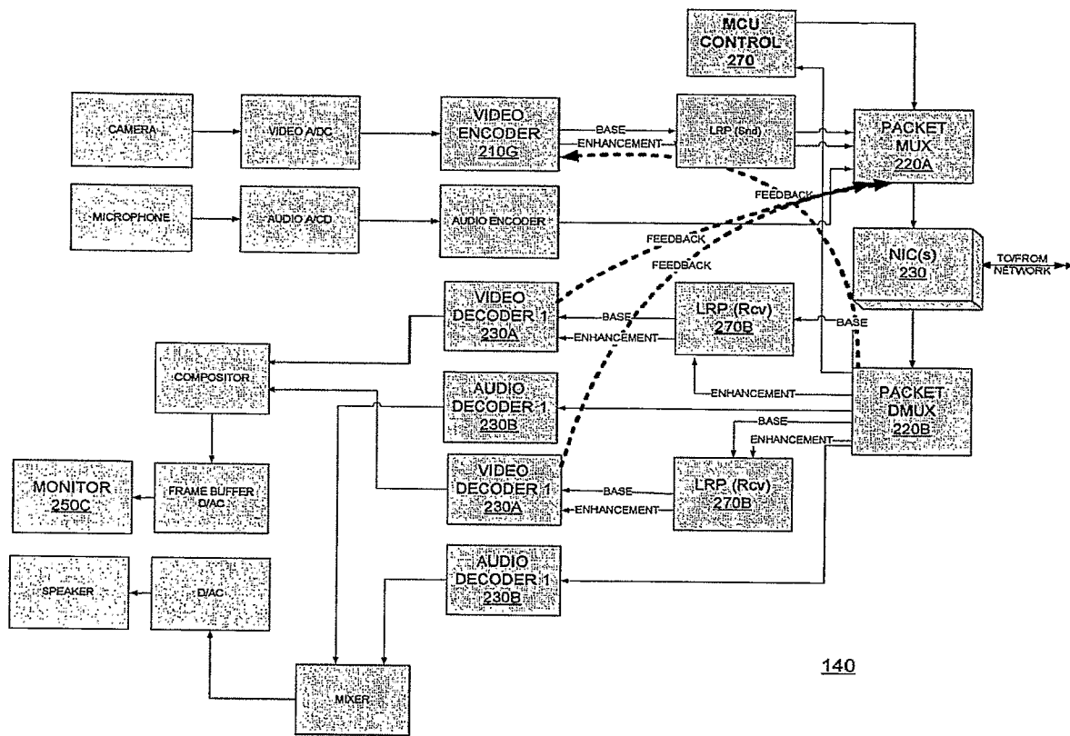
FIG. 3: END-USER TERMINAL (SCALABLE OR SIMULCAST CODING)
