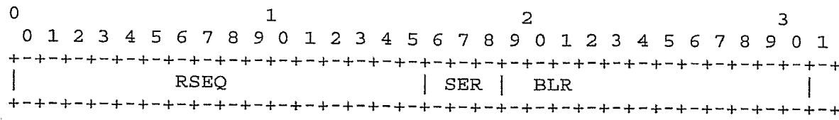
FIG. 20: RNACK FEEDBACK CONTROL INFORMATION (FCI) FIELD
