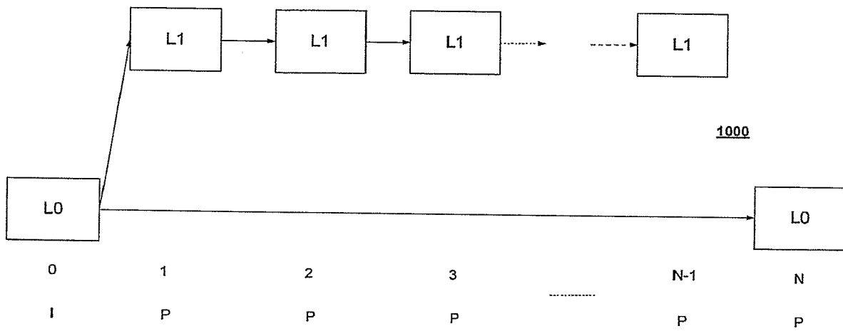
FIG. 10: ALTERNATIVE PICTURE CODING STRUCTURE EXAMPLE
