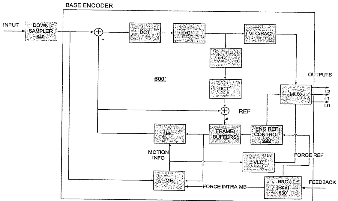
FIG. 7: VIDEO ENCODER (BASE AND TEMPORAL ENHANCEMENT LAYERS)
