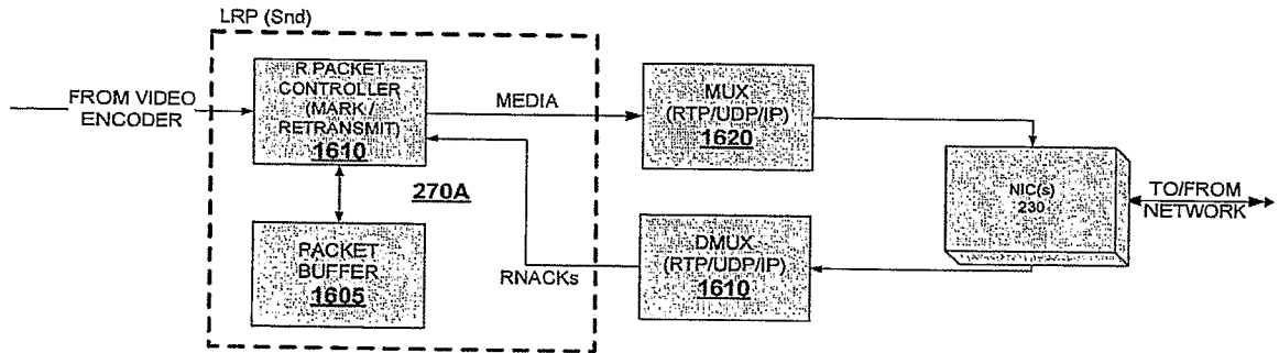
FIG. 16: TRANSMITTING TERMINAL WITH LRP USING RTP
