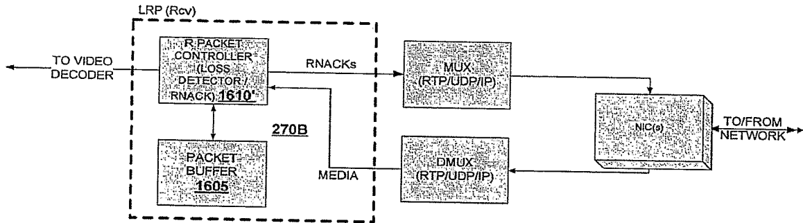
FIG. 17: RECEIVING TERMINAL WITH LRP USING RTP
