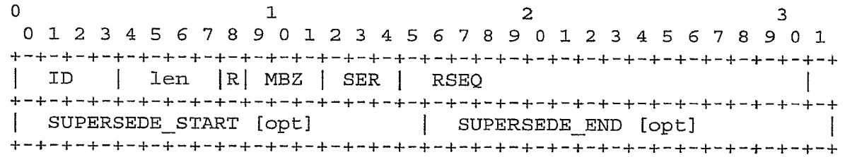
FIG. 19: RTP HEADER EXTENSION FOR RTP PACKETS
