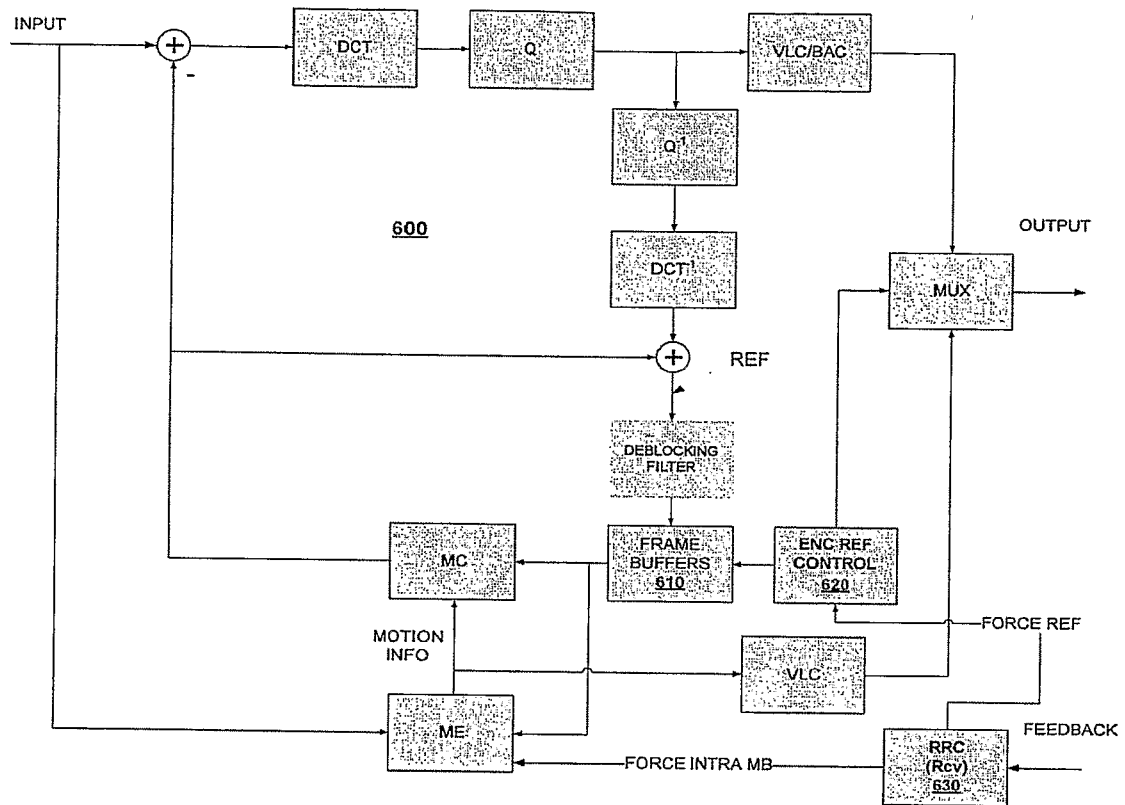
FIG. 6: VIDEO ENCODER
