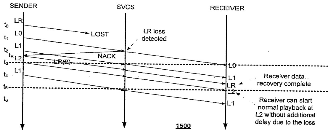
FIG. 15: THE LR PROTECTION (LRP) PROTOCOL USING NEGATIVE
