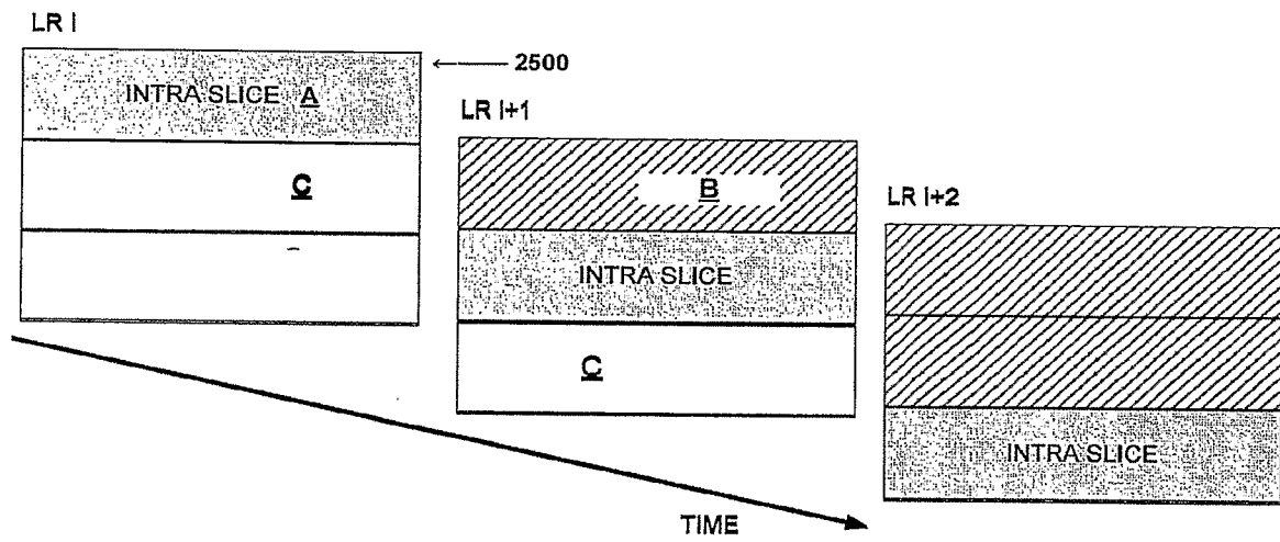
FIG. 25: FAST-FORWARD INTRA RECOVERY
