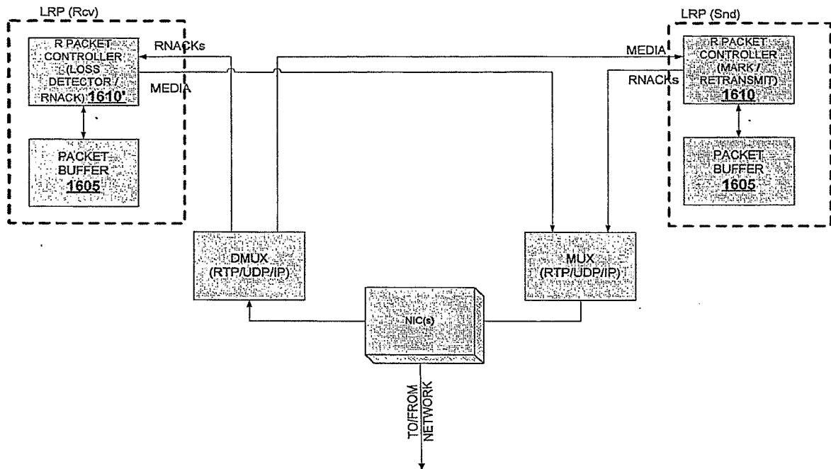
FIG. 18: SERVER WITH LRP USING RTP
