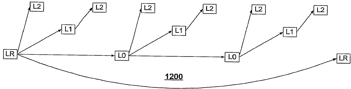
FIG. 12: PICTURE CODING STRUCTURE WITH LR PICTURES
