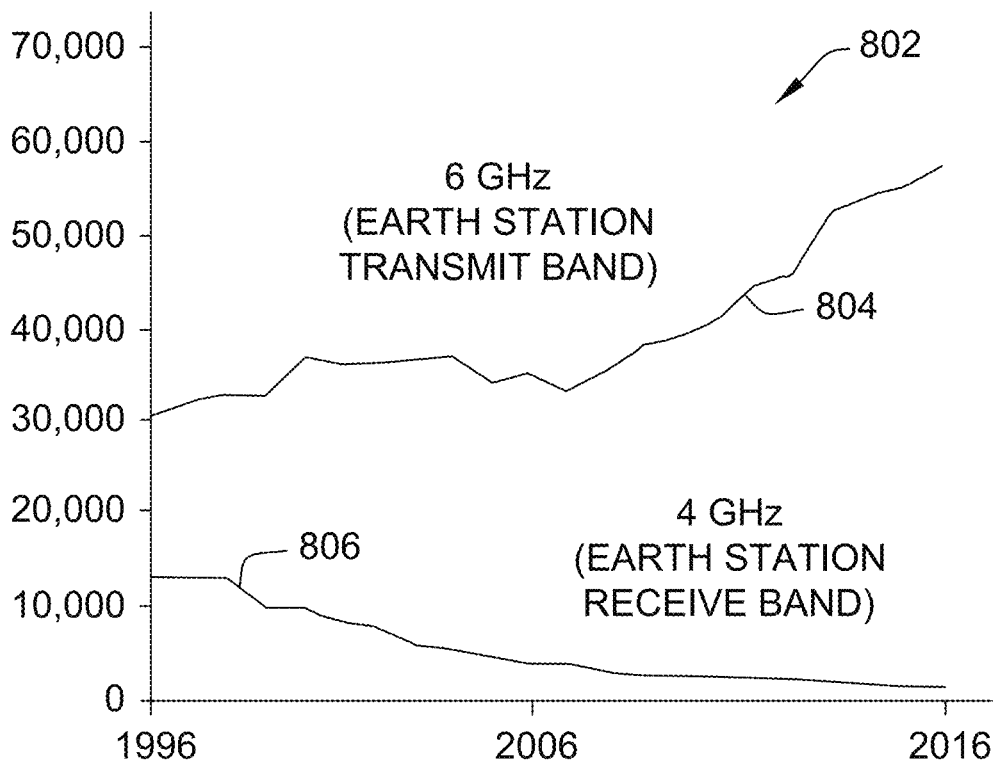
4 & 6 GHz FIXED MICROWAVE TIME TRENDS
