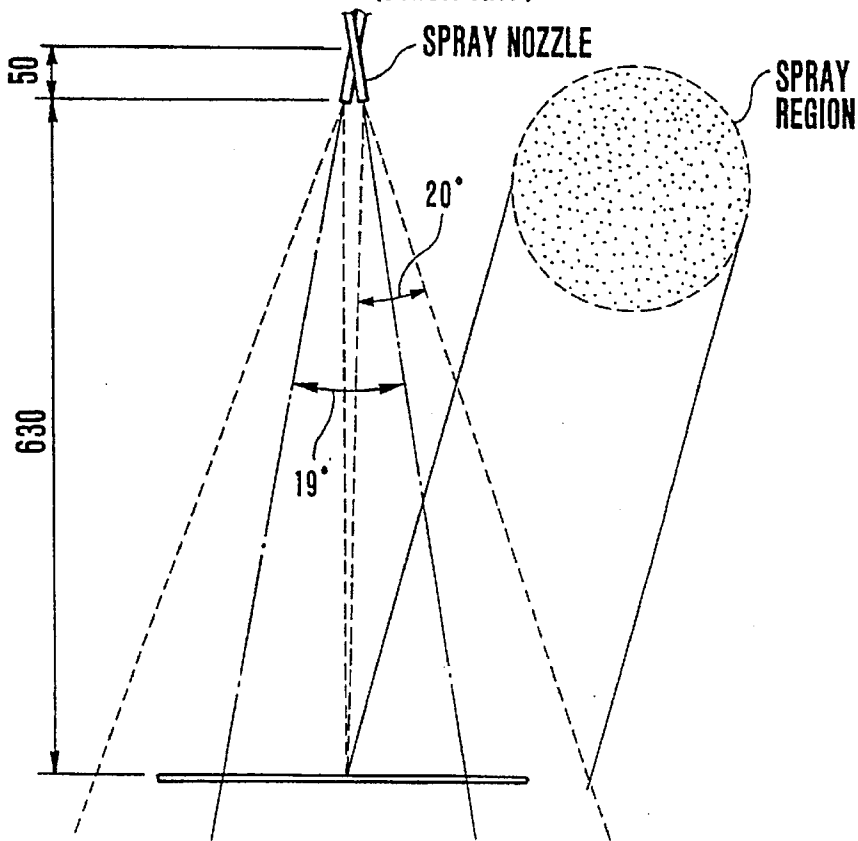
FIG.20 (PRIOR ART)
