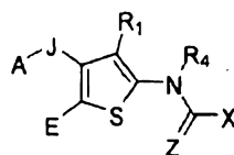
Formula (V);
