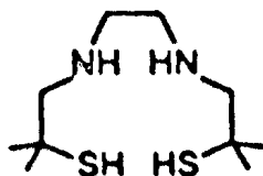
BAT N 2 S 2 diaminedithiol
