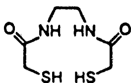
35 DADS N 2 S 2 diamidedithiol
