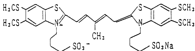
dye A
