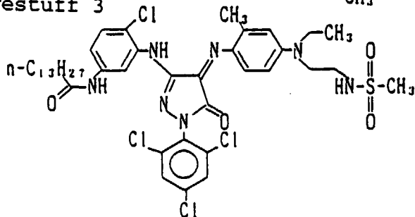
dyestuff 3
