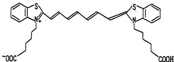
dyestuff 1
