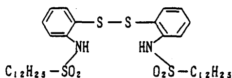
disulfide compound 1
