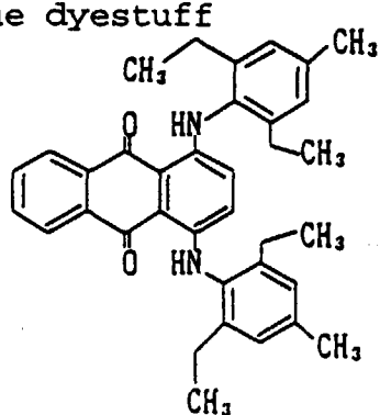
blue dyestuff
