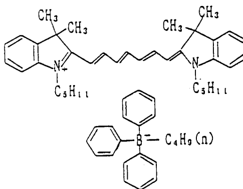
dyestuff A
