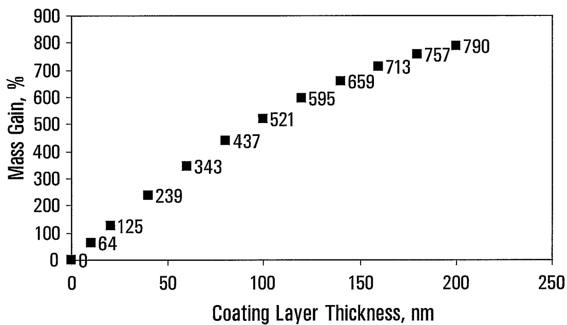
Theoretical Mass Gain as a Function of Coating Layer Thickness
