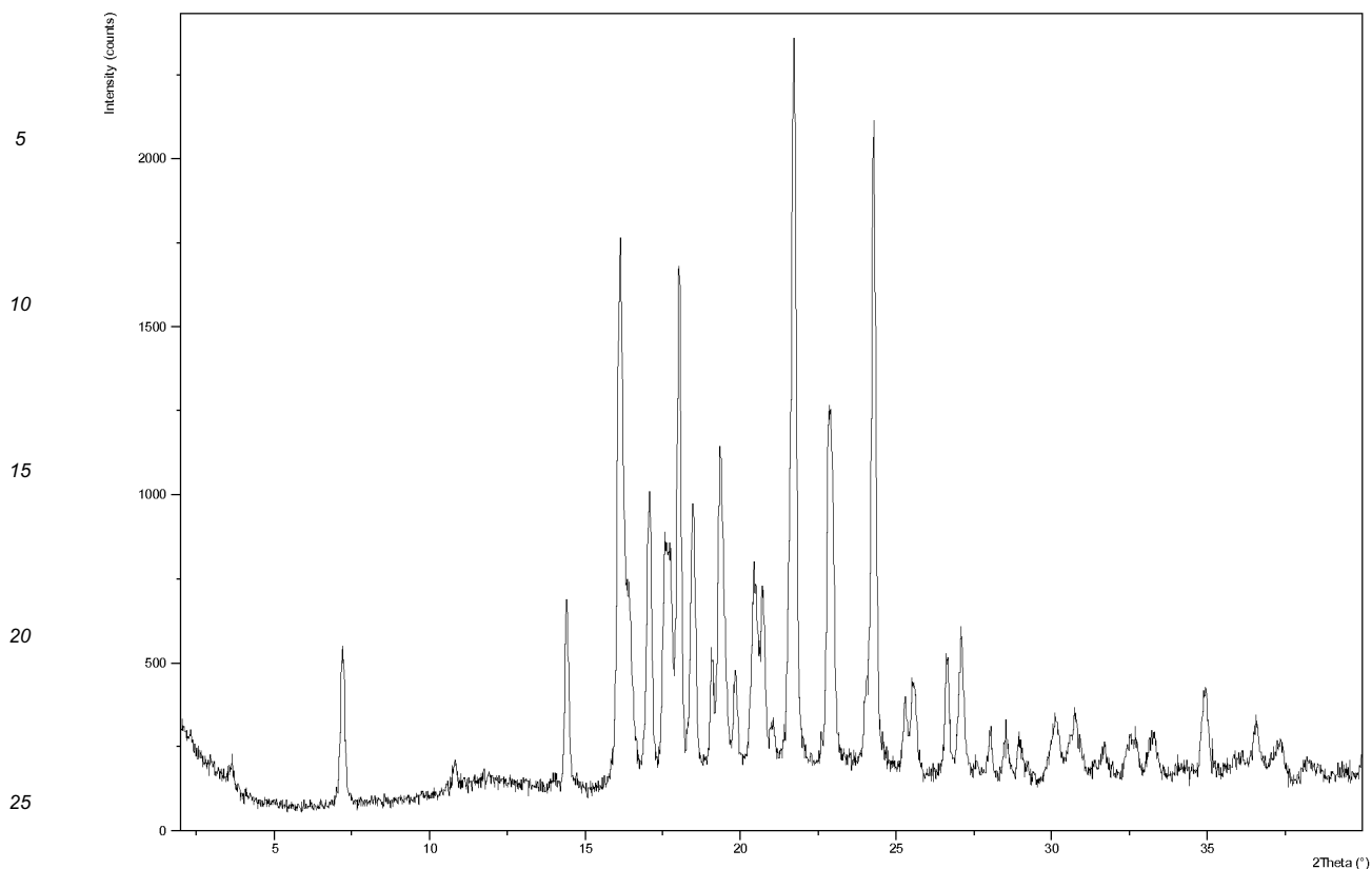
Figure 1: XRPD spectrum for compound of Formula (I)
