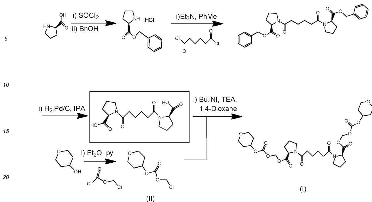
Reaction Scheme 2
