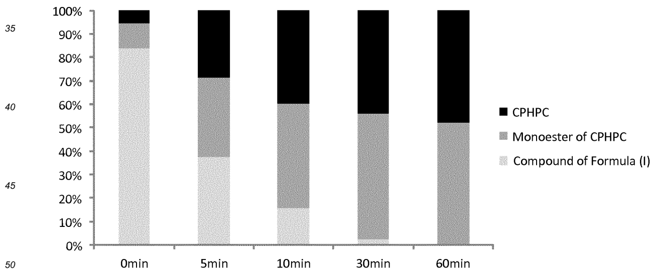
Figure 5: In vitro Liver microsomal stability of compound of Formula (I) in human liver microsomes. “0/5/10/30/60min” refers to the time (in minutes) that the sample was taken from the mixture for analysis.
