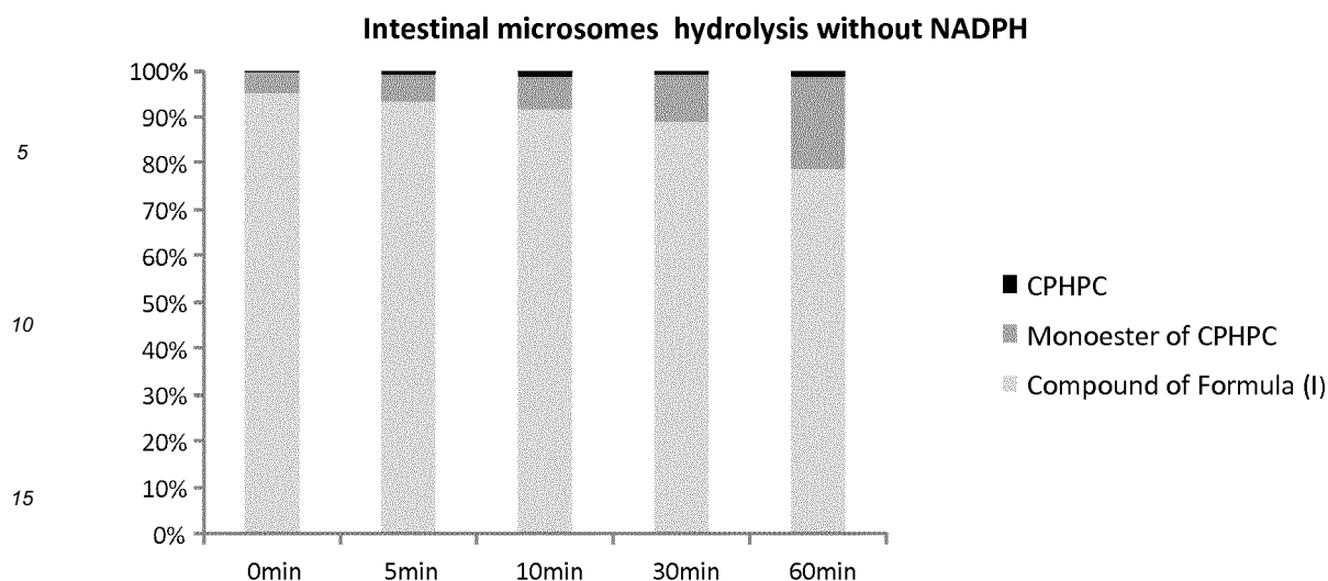
Figure 3: In vitro Intestinal Microsomal Stability of Compound of Formula (I) in human microsomes. "0/5/10/30/60min" refers to the time (in minutes) that the sample was taken from the mixture for analysis.
